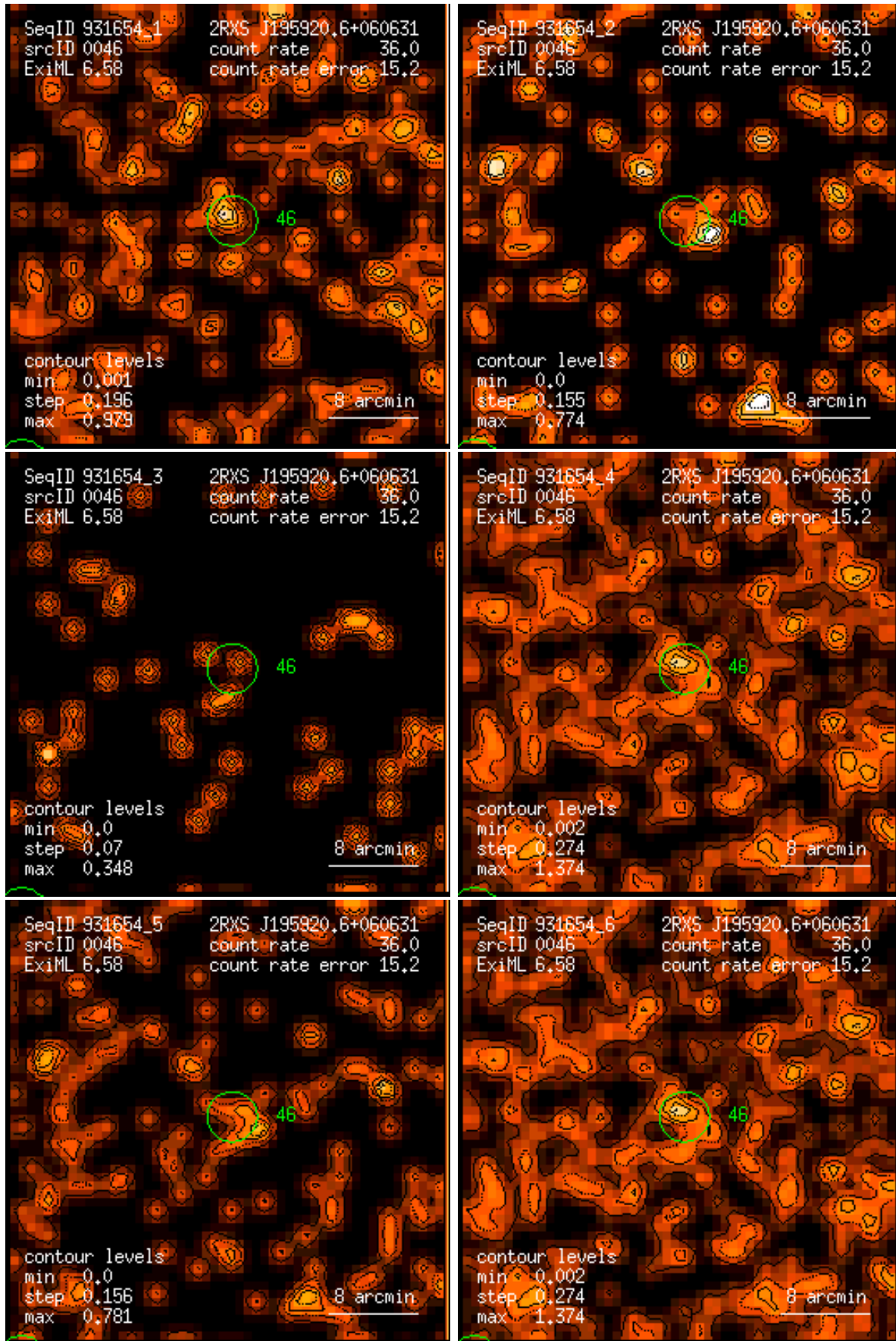
Figure 46: RASS 931654: detection 0046: band rate images, Gaussian filter: (1) PSPC channels 11 – 41, (2) 52 – 90, (3) 91 – 201, (4) 11 – 235, (5) 52 – 201, (6) 11 – 201. Broad band rates in counts/ks. Band rate contour levels in counts/ks/arcmin 2 .
