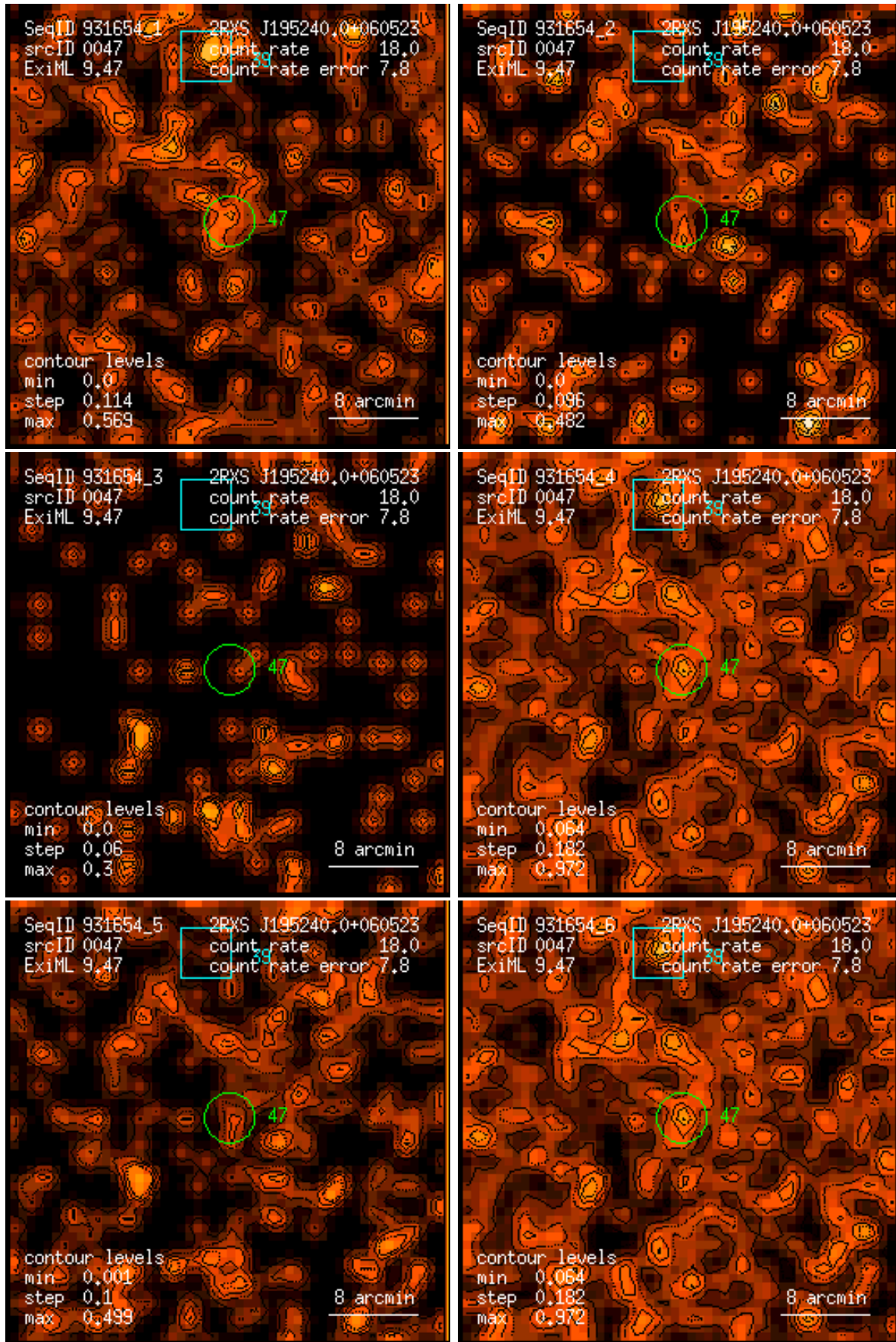
Figure 47: RASS 931654: detection 0047: band rate images, Gaussian filter: (1) PSPC channels 11 – 41, (2) 52 – 90, (3) 91 – 201, (4) 11 – 235, (5) 52 – 201, (6) 11 – 201. Broad band rates in counts/ks. Band rate contour levels in counts/ks/arcmin 2 .
