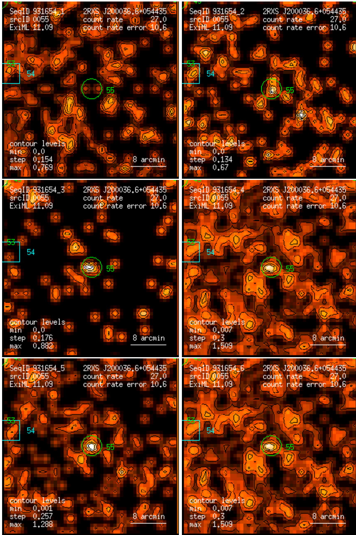
Figure 55: RASS 931654: detection 0055: band rate images, Gaussian filter: (1) PSPC channels 11 – 41, (2) 52 – 90, (3) 91 – 201, (4) 11 – 235, (5) 52 – 201, (6) 11 – 201. Broad band rates in counts/ks. Band rate contour levels in counts/ks/arcmin 2 .
