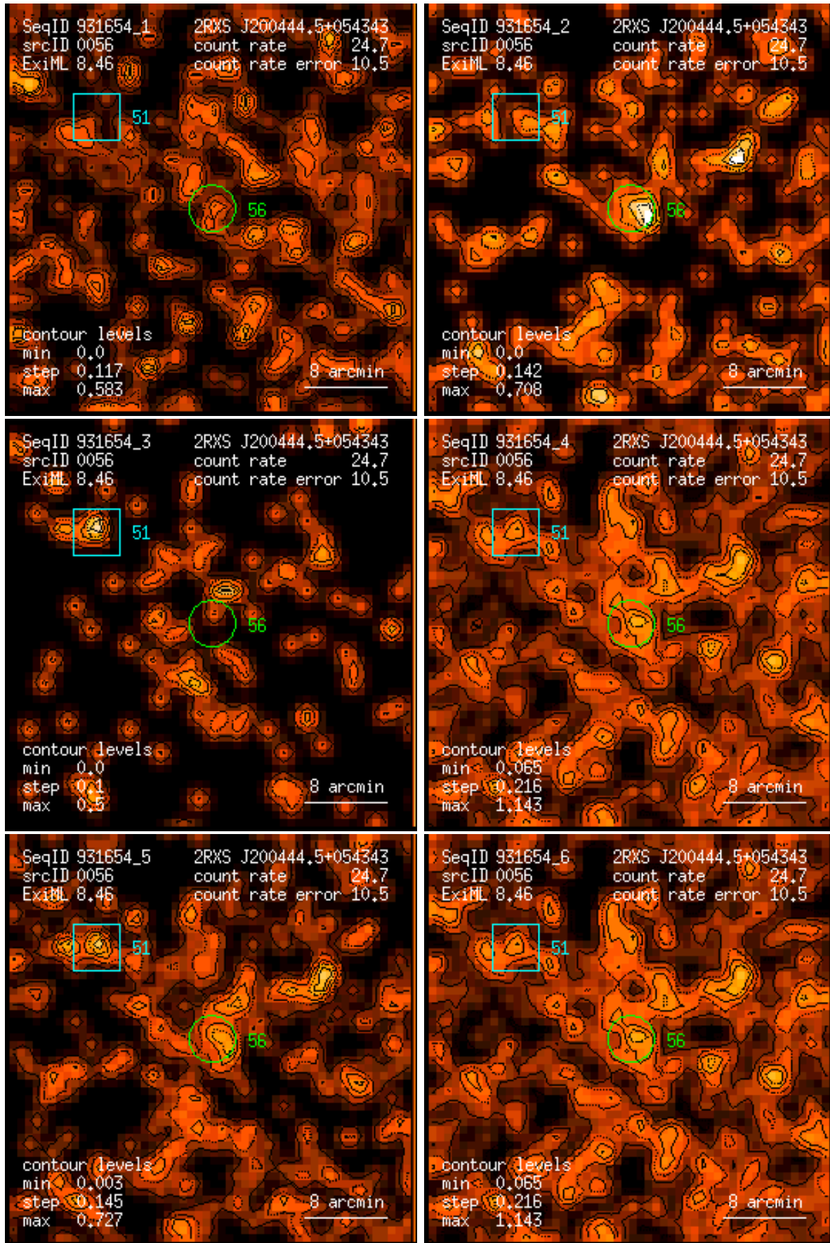
Figure 56: RASS 931654: detection 0056: band rate images, Gaussian filter: (1) PSPC channels 11 – 41, (2) 52 – 90, (3) 91 – 201, (4) 11 – 235, (5) 52 – 201, (6) 11 – 201. Broad band rates in counts/ks. Band rate contour levels in counts/ks/arcmin 2 .
