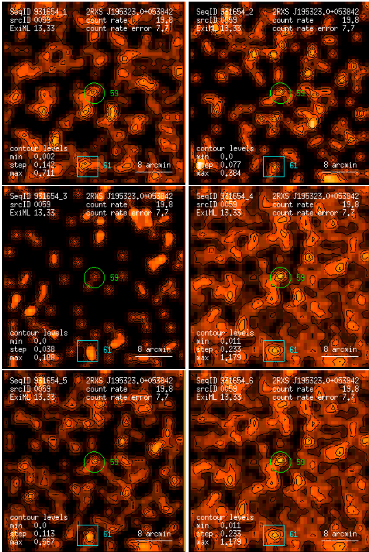
Figure 59: RASS 931654: detection 0059: band rate images, Gaussian filter: (1) PSPC channels 11 – 41, (2) 52 – 90, (3) 91 – 201, (4) 11 – 235, (5) 52 – 201, (6) 11 – 201. Broad band rates in counts/ks. Band rate contour levels in counts/ks/arcmin 2 .
