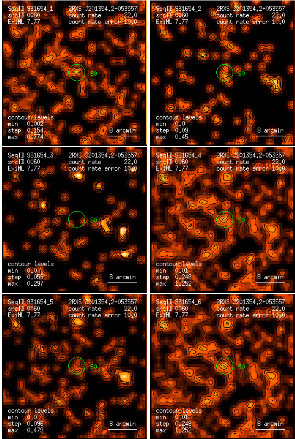
Figure 60: RASS 931654: detection 0060: band rate images, Gaussian filter: (1) PSPC channels 11 – 41, (2) 52 – 90, (3) 91 – 201, (4) 11 – 235, (5) 52 – 201, (6) 11 – 201. Broad band rates in counts/ks. Band rate contour levels in counts/ks/arcmin 2 .
