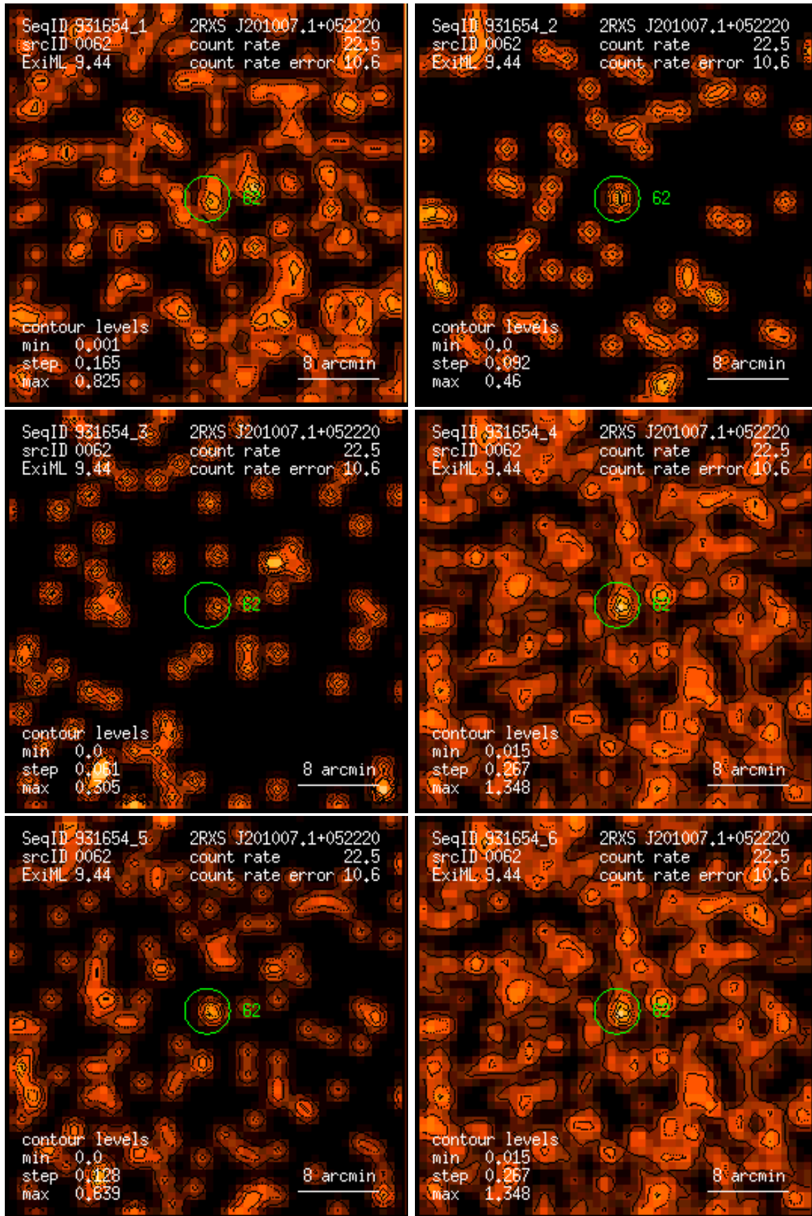
Figure 62: RASS 931654: detection 0062: band rate images, Gaussian filter: (1) PSPC channels 11 – 41, (2) 52 – 90, (3) 91 – 201, (4) 11 – 235, (5) 52 – 201, (6) 11 – 201. Broad band rates in counts/ks. Band rate contour levels in counts/ks/arcmin 2 .
