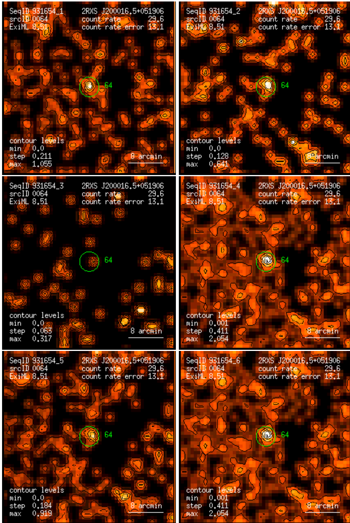
Figure 64: RASS 931654: detection 0064: band rate images, Gaussian filter: (1) PSPC channels 11 – 41, (2) 52 – 90, (3) 91 – 201, (4) 11 – 235, (5) 52 – 201, (6) 11 – 201. Broad band rates in counts/ks. Band rate contour levels in counts/ks/arcmin 2 .
