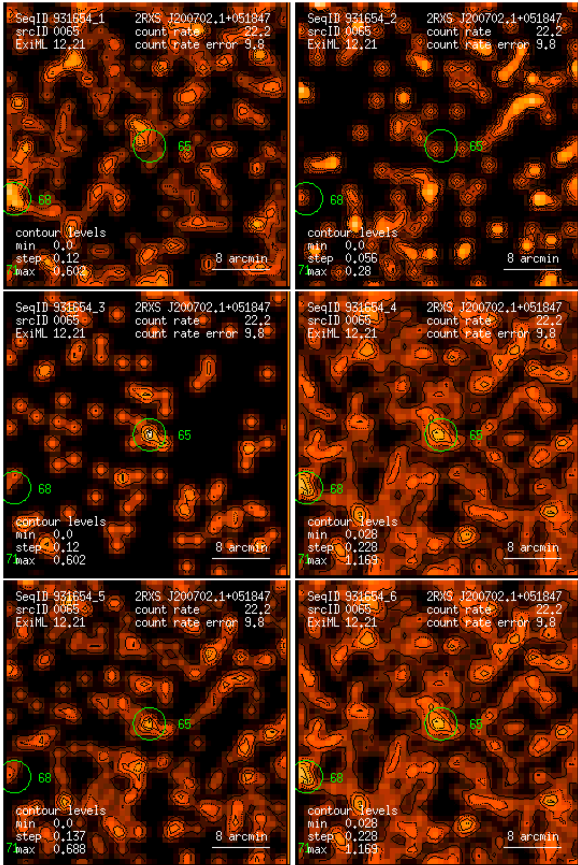
Figure 65: RASS 931654: detection 0065: band rate images, Gaussian filter: (1) PSPC channels 11 – 41, (2) 52 – 90, (3) 91 – 201, (4) 11 – 235, (5) 52 – 201, (6) 11 – 201. Broad band rates in counts/ks. Band rate contour levels in counts/ks/arcmin 2 .
