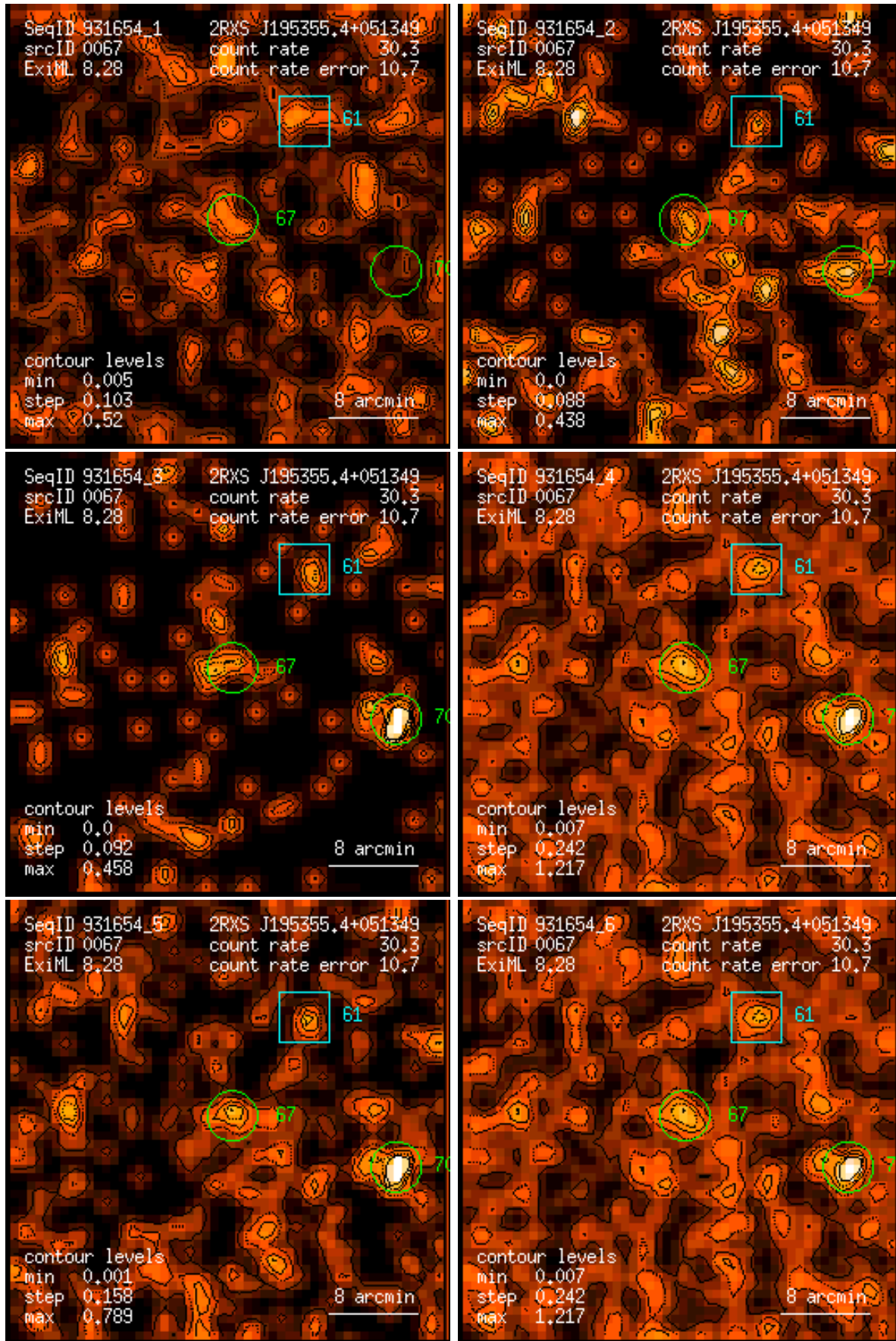
Figure 67: RASS 931654: detection 0067: band rate images, Gaussian filter: (1) PSPC channels 11 – 41, (2) 52 – 90, (3) 91 – 201, (4) 11 – 235, (5) 52 – 201, (6) 11 – 201. Broad band rates in counts/ks. Band rate contour levels in counts/ks/arcmin 2 .
