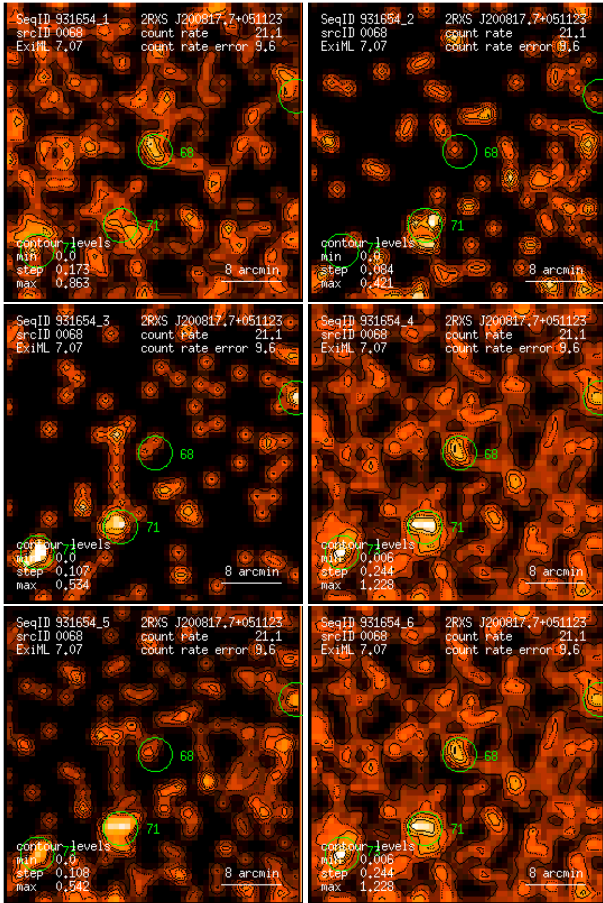
Figure 68: RASS 931654: detection 0068: band rate images, Gaussian filter: (1) PSPC channels 11 – 41, (2) 52 – 90, (3) 91 – 201, (4) 11 – 235, (5) 52 – 201, (6) 11 – 201. Broad band rates in counts/ks. Band rate contour levels in counts/ks/arcmin 2 .
