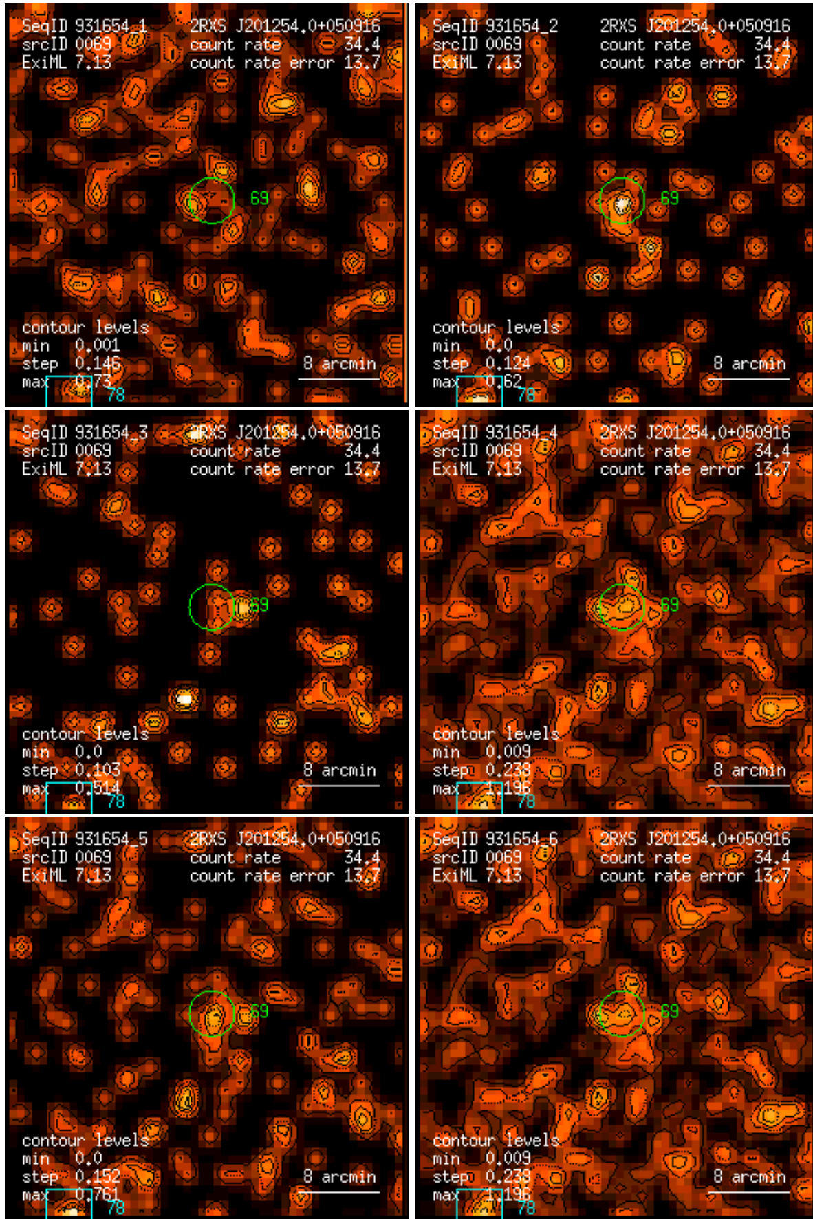
Figure 69: RASS 931654: detection 0069: band rate images, Gaussian filter: (1) PSPC channels 11 – 41, (2) 52 – 90, (3) 91 – 201, (4) 11 – 235, (5) 52 – 201, (6) 11 – 201. Broad band rates in counts/ks. Band rate contour levels in counts/ks/arcmin 2 .
