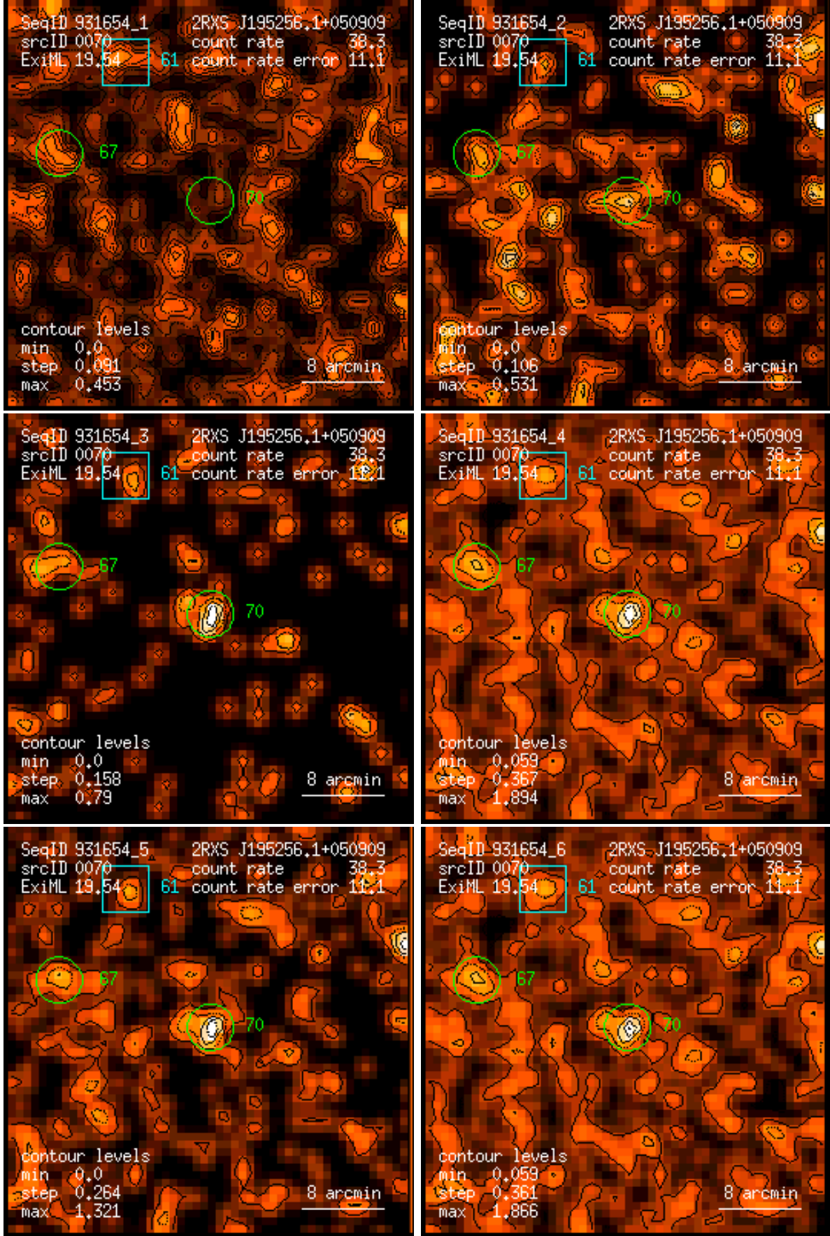
Figure 70: RASS 931654: detection 0070: band rate images, Gaussian filter: (1) PSPC channels 11 – 41, (2) 52 – 90, (3) 91 – 201, (4) 11 – 235, (5) 52 – 201, (6) 11 – 201. Broad band rates in counts/ks. Band rate contour levels in counts/ks/arcmin 2 .
