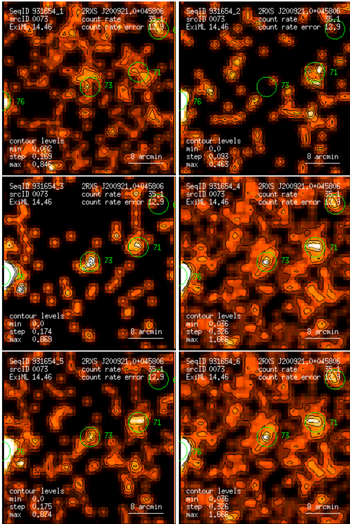
Figure 73: RASS 931654: detection 0073: band rate images, Gaussian filter: (1) PSPC channels 11 – 41, (2) 52 – 90, (3) 91 – 201, (4) 11 – 235, (5) 52 – 201, (6) 11 – 201. Broad band rates in counts/ks. Band rate contour levels in counts/ks/arcmin 2 .
