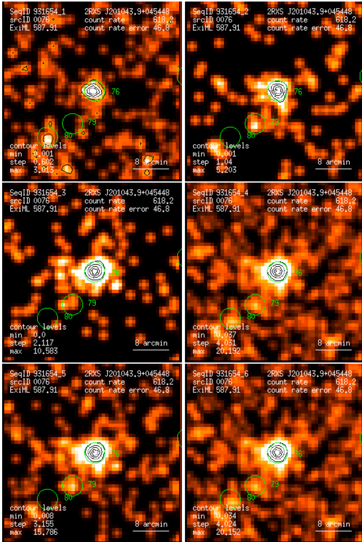
Figure 76: RASS 931654: detection 0076: band rate images, Gaussian filter: (1) PSPC channels 11 – 41, (2) 52 – 90, (3) 91 – 201, (4) 11 – 235, (5) 52 – 201, (6) 11 – 201. Broad band rates in counts/ks. Band rate contour levels in counts/ks/arcmin 2 .
