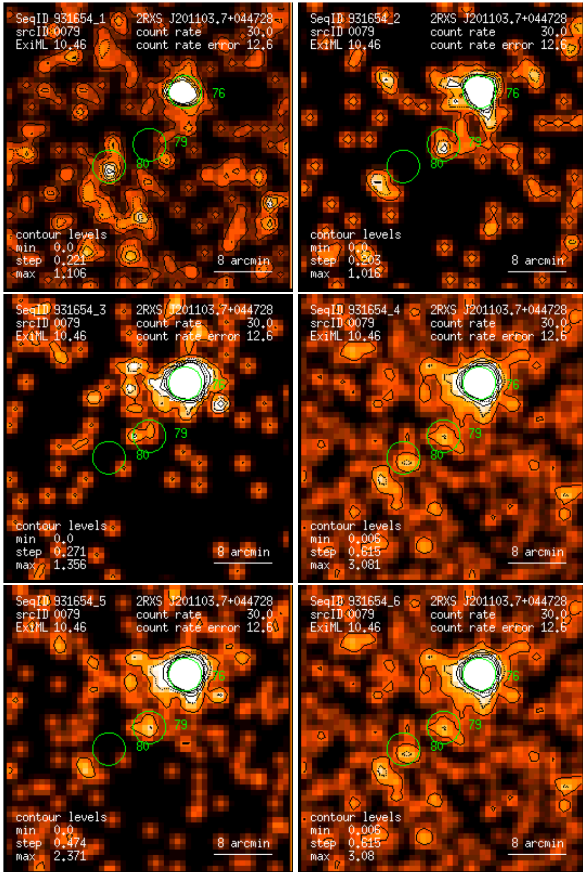
Figure 79: RASS 931654: detection 0079: band rate images, Gaussian filter: (1) PSPC channels 11 – 41, (2) 52 – 90, (3) 91 – 201, (4) 11 – 235, (5) 52 – 201, (6) 11 – 201. Broad band rates in counts/ks. Band rate contour levels in counts/ks/arcmin 2 .
