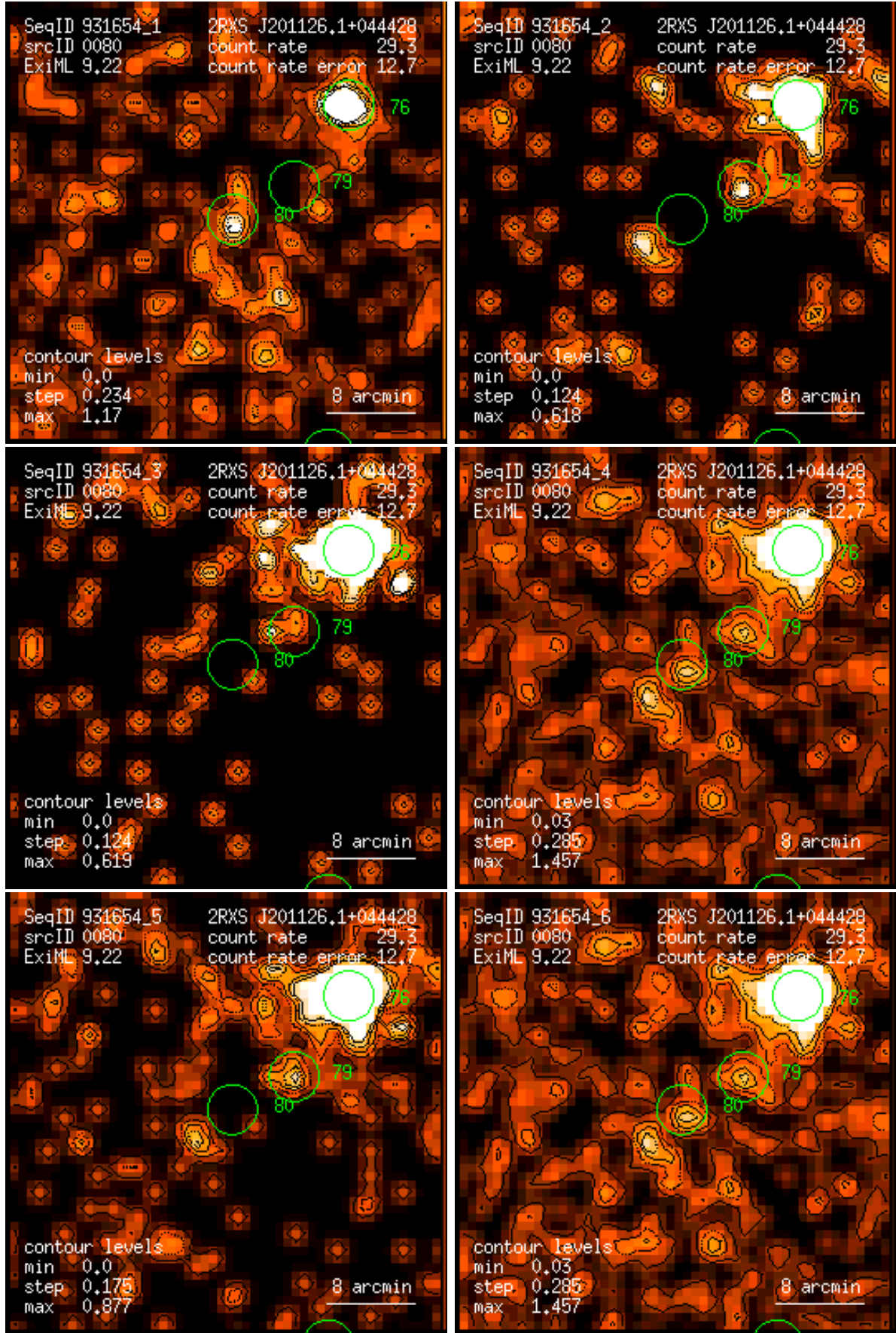
Figure 80: RASS 931654: detection 0080: band rate images, Gaussian filter: (1) PSPC channels 11 – 41, (2) 52 – 90, (3) 91 – 201, (4) 11 – 235, (5) 52 – 201, (6) 11 – 201. Broad band rates in counts/ks. Band rate contour levels in counts/ks/arcmin 2 .
