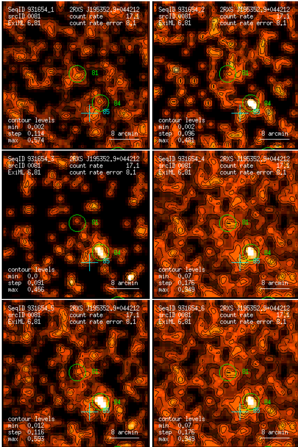
Figure 81: RASS 931654: detection 0081: band rate images, Gaussian filter: (1) PSPC channels 11 – 41, (2) 52 – 90, (3) 91 – 201, (4) 11 – 235, (5) 52 – 201, (6) 11 – 201. Broad band rates in counts/ks. Band rate contour levels in counts/ks/arcmin 2 .
