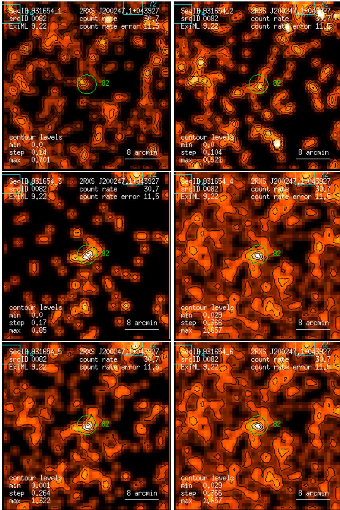
Figure 82: RASS 931654: detection 0082: band rate images, Gaussian filter: (1) PSPC channels 11 – 41, (2) 52 – 90, (3) 91 – 201, (4) 11 – 235, (5) 52 – 201, (6) 11 – 201. Broad band rates in counts/ks. Band rate contour levels in counts/ks/arcmin 2 .
