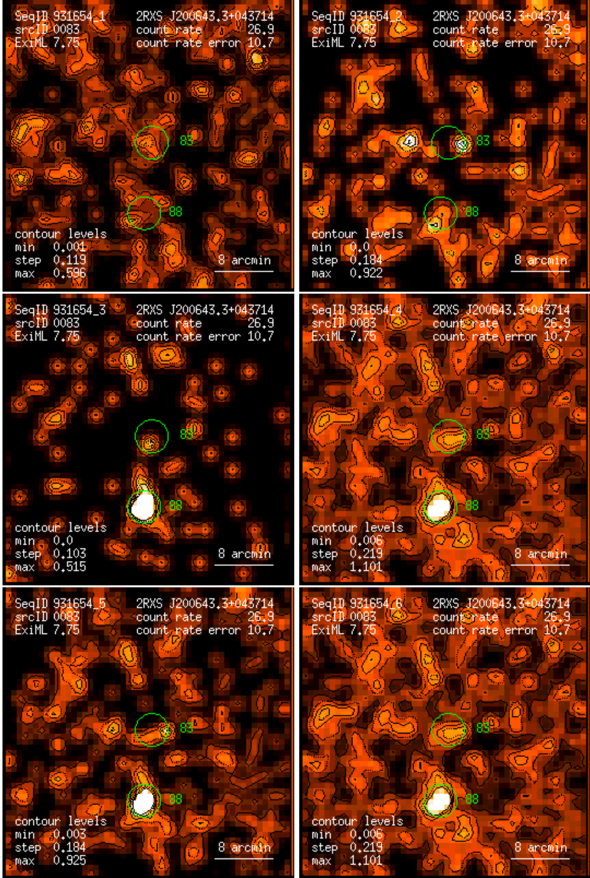
Figure 83: RASS 931654: detection 0083: band rate images, Gaussian filter: (1) PSPC channels 11 – 41, (2) 52 – 90, (3) 91 – 201, (4) 11 – 235, (5) 52 – 201, (6) 11 – 201. Broad band rates in counts/ks. Band rate contour levels in counts/ks/arcmin 2 .
