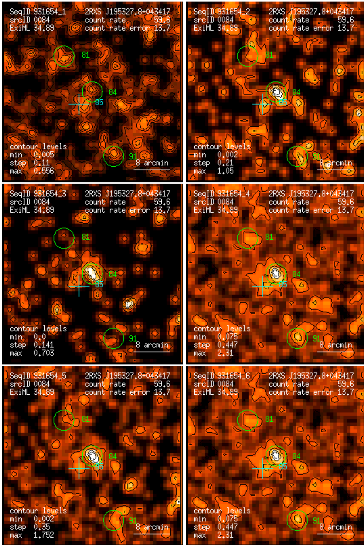
Figure 84: RASS 931654: detection 0084: band rate images, Gaussian filter: (1) PSPC channels 11 – 41, (2) 52 – 90, (3) 91 – 201, (4) 11 – 235, (5) 52 – 201, (6) 11 – 201. Broad band rates in counts/ks. Band rate contour levels in counts/ks/arcmin 2 .
