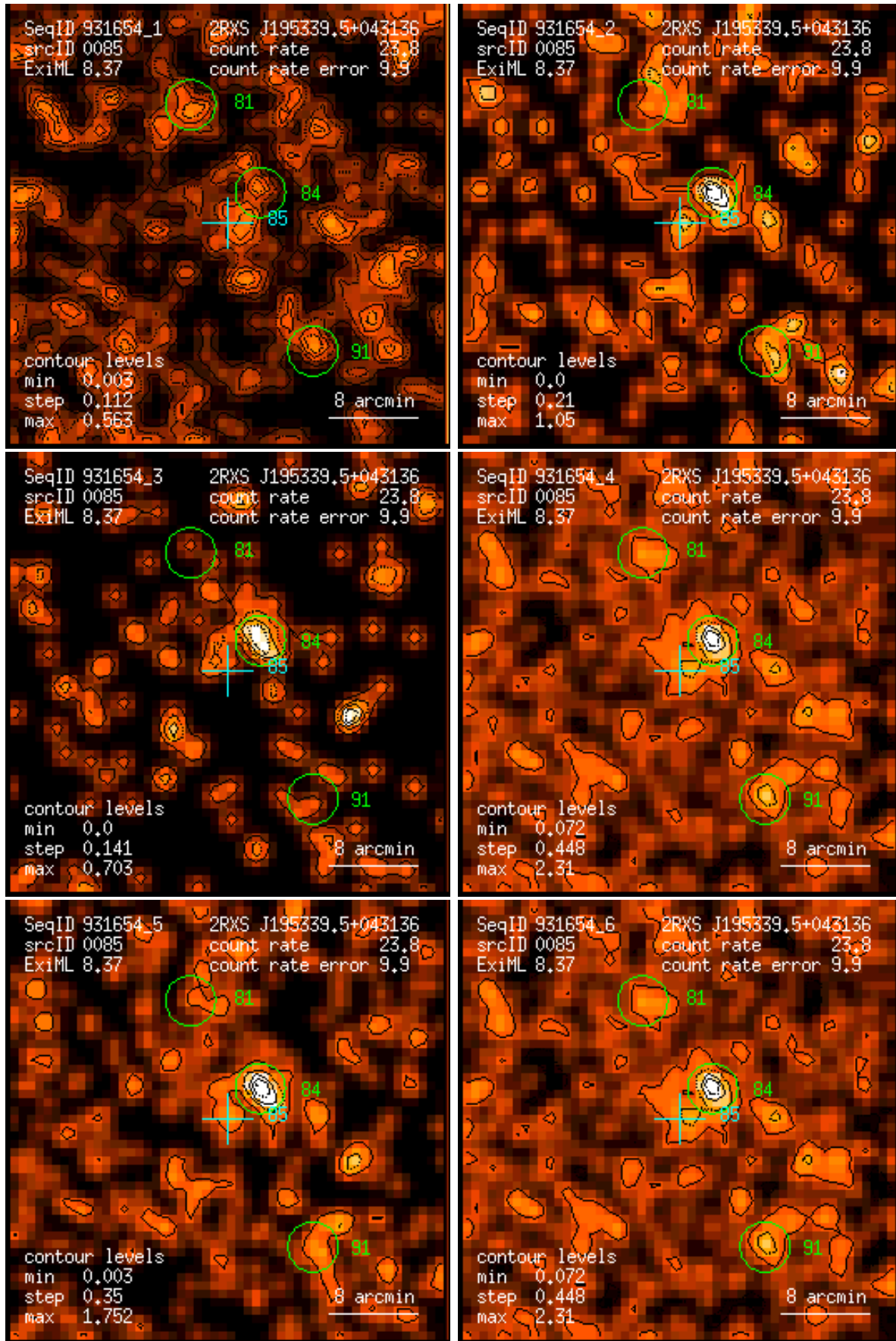
Figure 85: RASS 931654: detection 0085: band rate images, Gaussian filter: (1) PSPC channels 11 – 41, (2) 52 – 90, (3) 91 – 201, (4) 11 – 235, (5) 52 – 201, (6) 11 – 201. Broad band rates in counts/ks. Band rate contour levels in counts/ks/arcmin 2 .
