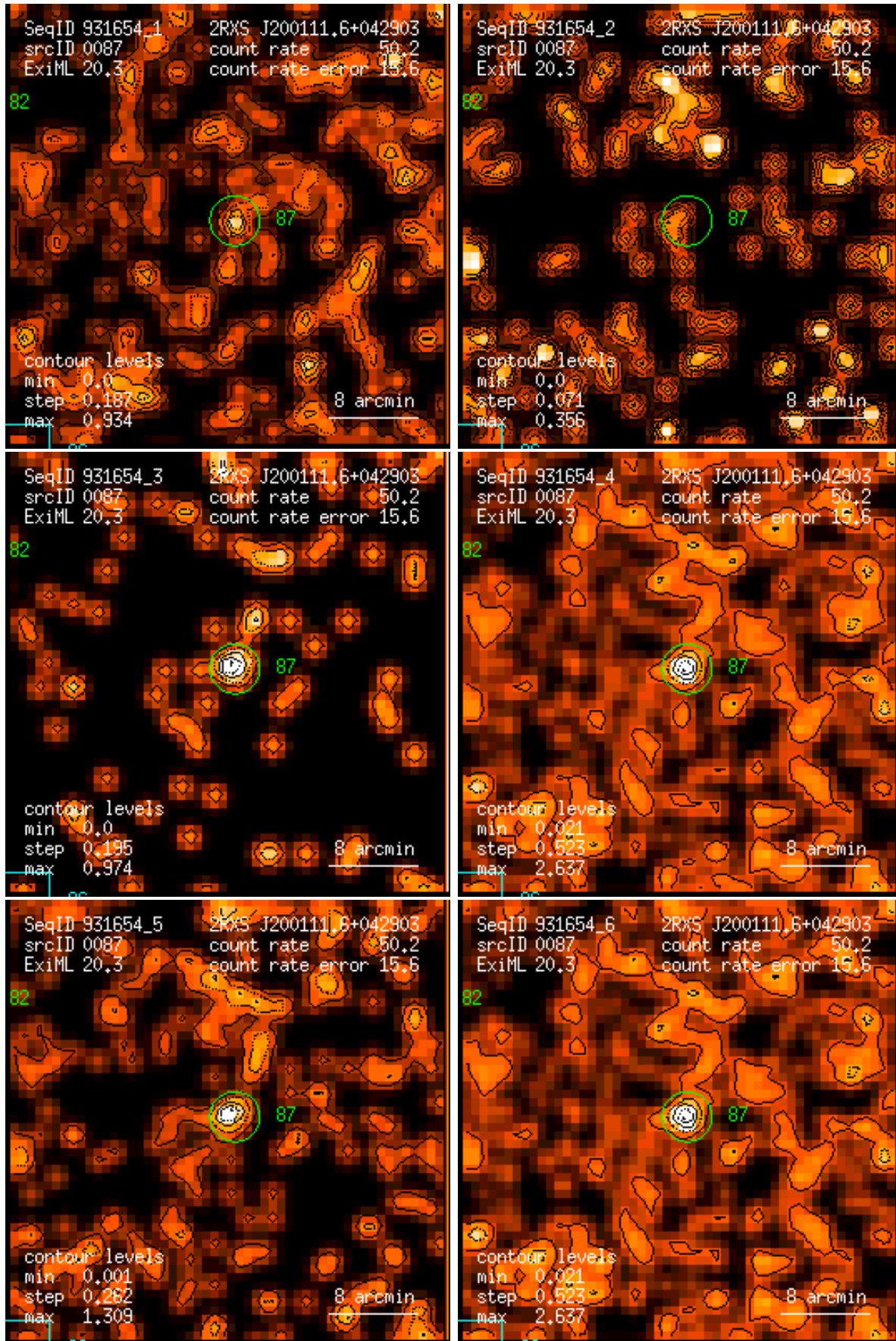
Figure 87: RASS 931654: detection 0087: band rate images, Gaussian filter: (1) PSPC channels 11 – 41, (2) 52 – 90, (3) 91 – 201, (4) 11 – 235, (5) 52 – 201, (6) 11 – 201. Broad band rates in counts/ks. Band rate contour levels in counts/ks/arcmin 2 .
