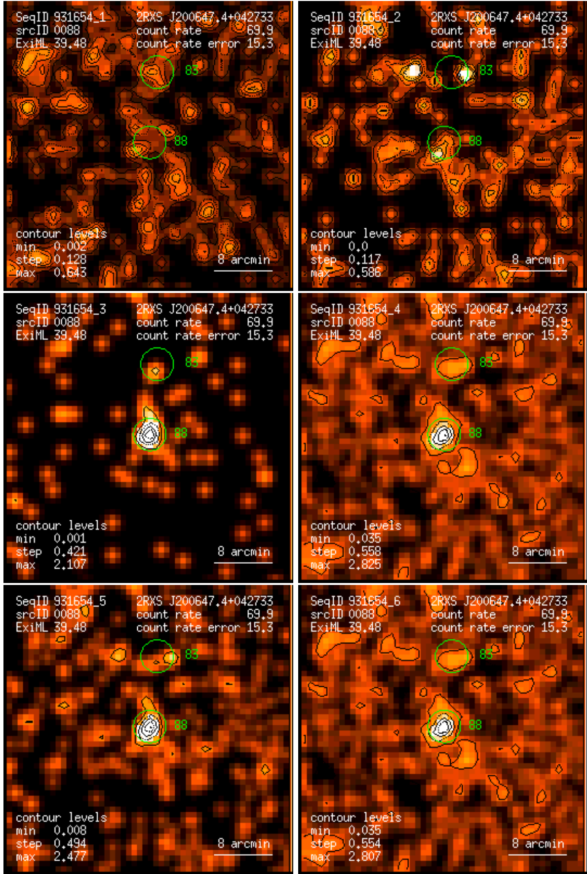
Figure 88: RASS 931654: detection 0088: band rate images, Gaussian filter: (1) PSPC channels 11 – 41, (2) 52 – 90, (3) 91 – 201, (4) 11 – 235, (5) 52 – 201, (6) 11 – 201. Broad band rates in counts/ks. Band rate contour levels in counts/ks/arcmin 2 .
