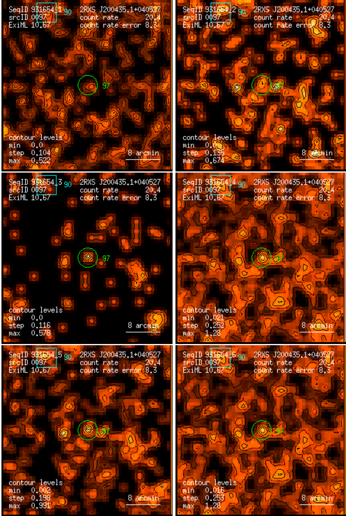
Figure 97: RASS 931654: detection 0097: band rate images, Gaussian filter: (1) PSPC channels 11 – 41, (2) 52 – 90, (3) 91 – 201, (4) 11 – 235, (5) 52 – 201, (6) 11 – 201. Broad band rates in counts/ks. Band rate contour levels in counts/ks/arcmin 2 .
