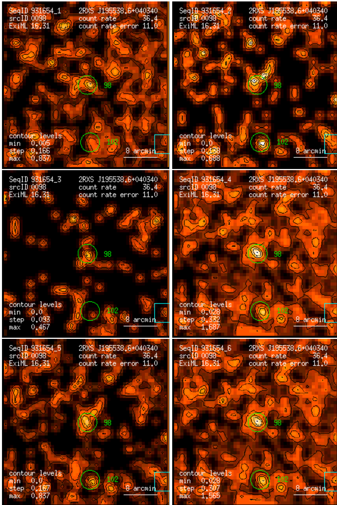
Figure 98: RASS 931654: detection 0098: band rate images, Gaussian filter: (1) PSPC channels 11 – 41, (2) 52 – 90, (3) 91 – 201, (4) 11 – 235, (5) 52 – 201, (6) 11 – 201. Broad band rates in counts/ks. Band rate contour levels in counts/ks/arcmin 2 .
