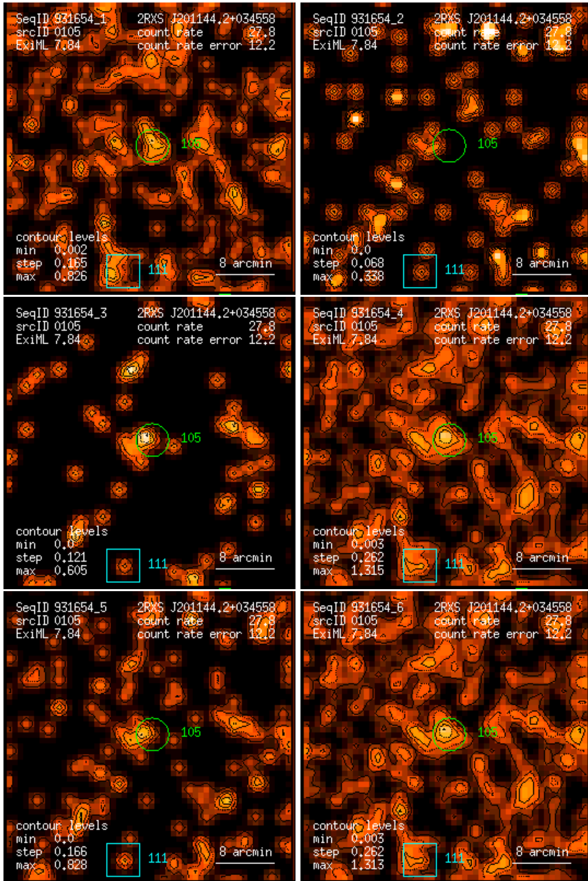
Figure 105: RASS 931654: detection 0105: band rate images, Gaussian filter: (1) PSPC channels 11 – 41, (2) 52 – 90, (3) 91 – 201, (4) 11 – 235, (5) 52 – 201, (6) 11 – 201. Broad band rates in counts/ks. Band rate contour levels in counts/ks/arcmin 2 .
