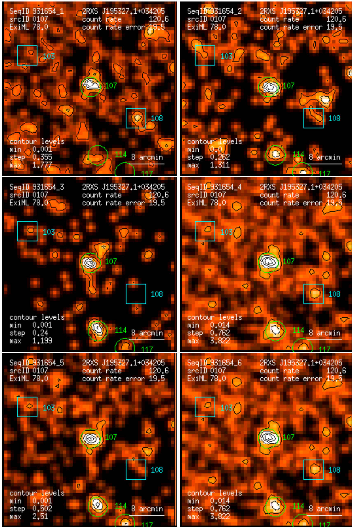
Figure 107: RASS 931654: detection 0107: band rate images, Gaussian filter: (1) PSPC channels 11 – 41, (2) 52 – 90, (3) 91 – 201, (4) 11 – 235, (5) 52 – 201, (6) 11 – 201. Broad band rates in counts/ks. Band rate contour levels in counts/ks/arcmin 2 .
