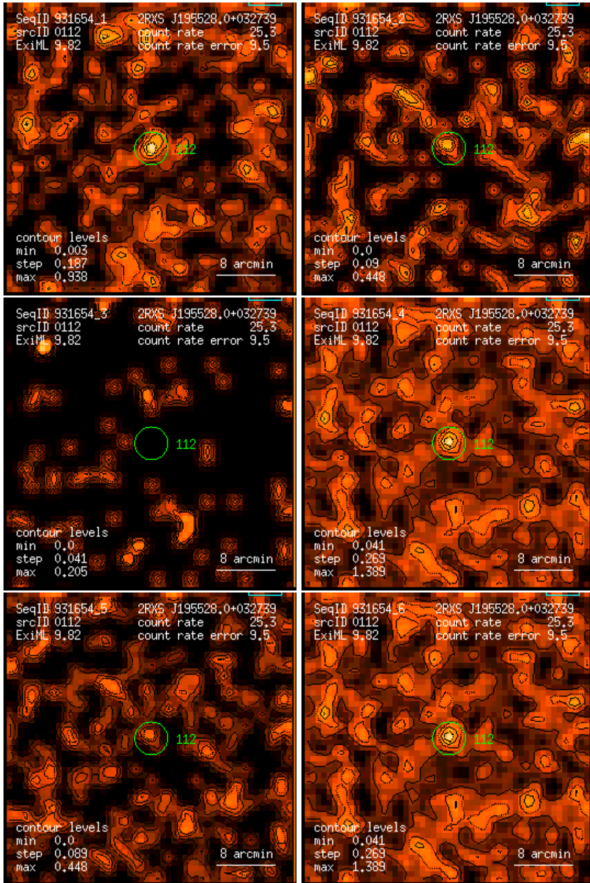
Figure 112: RASS 931654: detection 0112: band rate images, Gaussian filter: (1) PSPC channels 11 – 41, (2) 52 – 90, (3) 91 – 201, (4) 11 – 235, (5) 52 – 201, (6) 11 – 201. Broad band rates in counts/ks. Band rate contour levels in counts/ks/arcmin 2 .
