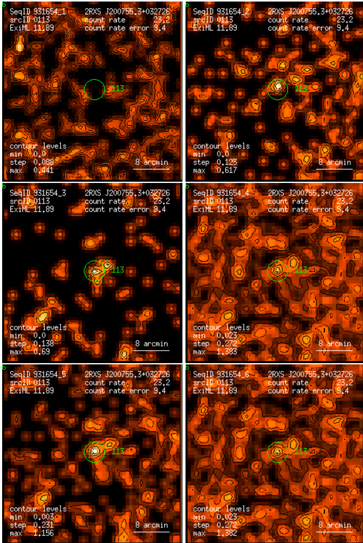
Figure 113: RASS 931654: detection 0113: band rate images, Gaussian filter: (1) PSPC channels 11 – 41, (2) 52 – 90, (3) 91 – 201, (4) 11 – 235, (5) 52 – 201, (6) 11 – 201. Broad band rates in counts/ks. Band rate contour levels in counts/ks/arcmin 2 .
