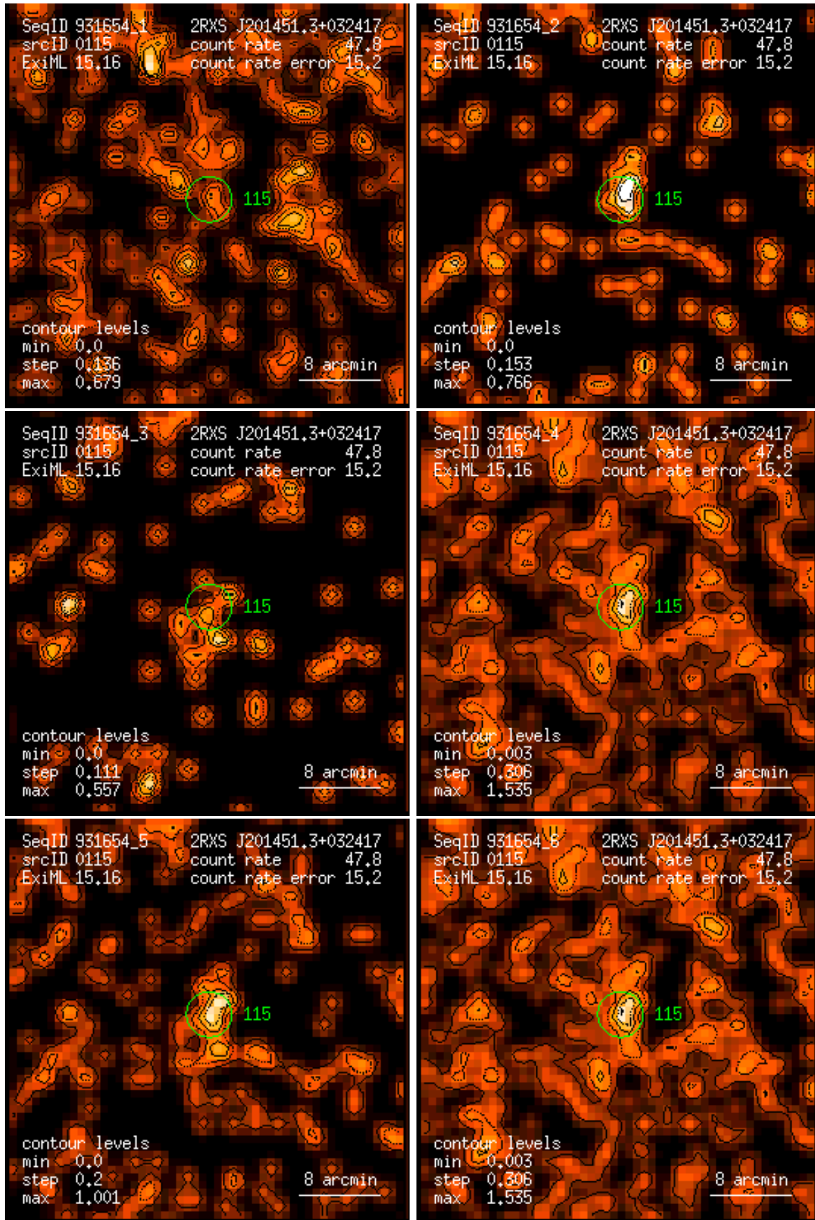
Figure 115: RASS 931654: detection 0115: band rate images, Gaussian filter: (1) PSPC channels 11 – 41, (2) 52 – 90, (3) 91 – 201, (4) 11 – 235, (5) 52 – 201, (6) 11 – 201. Broad band rates in counts/ks. Band rate contour levels in counts/ks/arcmin 2 .
