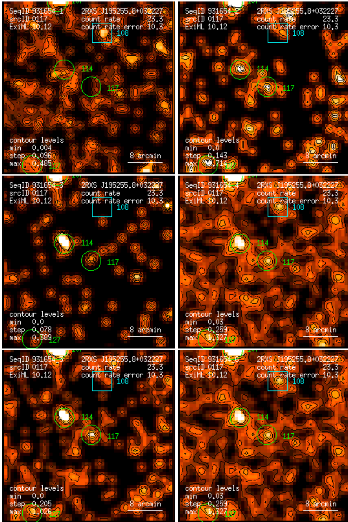
Figure 117: RASS 931654: detection 0117: band rate images, Gaussian filter: (1) PSPC channels 11 – 41, (2) 52 – 90, (3) 91 – 201, (4) 11 – 235, (5) 52 – 201, (6) 11 – 201. Broad band rates in counts/ks. Band rate contour levels in counts/ks/arcmin 2 .
