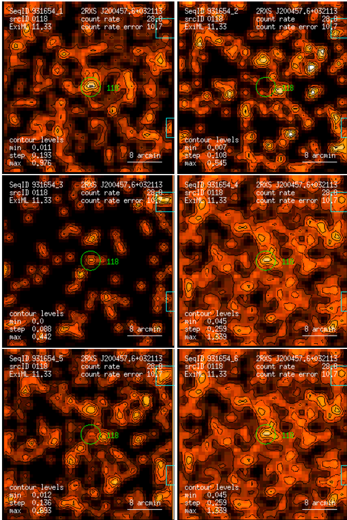
Figure 118: RASS 931654: detection 0118: band rate images, Gaussian filter: (1) PSPC channels 11 – 41, (2) 52 – 90, (3) 91 – 201, (4) 11 – 235, (5) 52 – 201, (6) 11 – 201. Broad band rates in counts/ks. Band rate contour levels in counts/ks/arcmin 2 .
