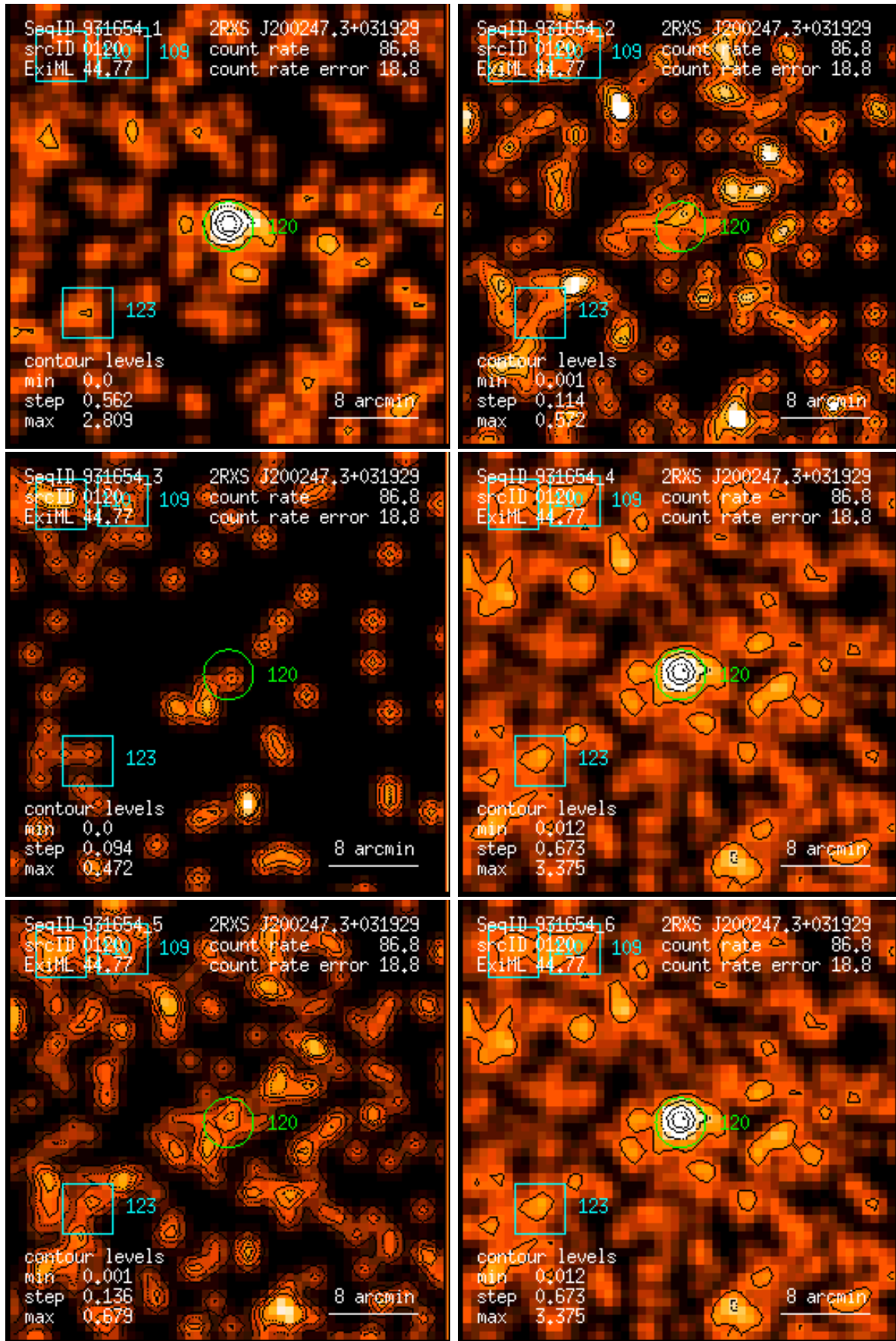
Figure 120: RASS 931654: detection 0120: band rate images, Gaussian filter: (1) PSPC channels 11 – 41, (2) 52 – 90, (3) 91 – 201, (4) 11 – 235, (5) 52 – 201, (6) 11 – 201. Broad band rates in counts/ks. Band rate contour levels in counts/ks/arcmin 2 .
