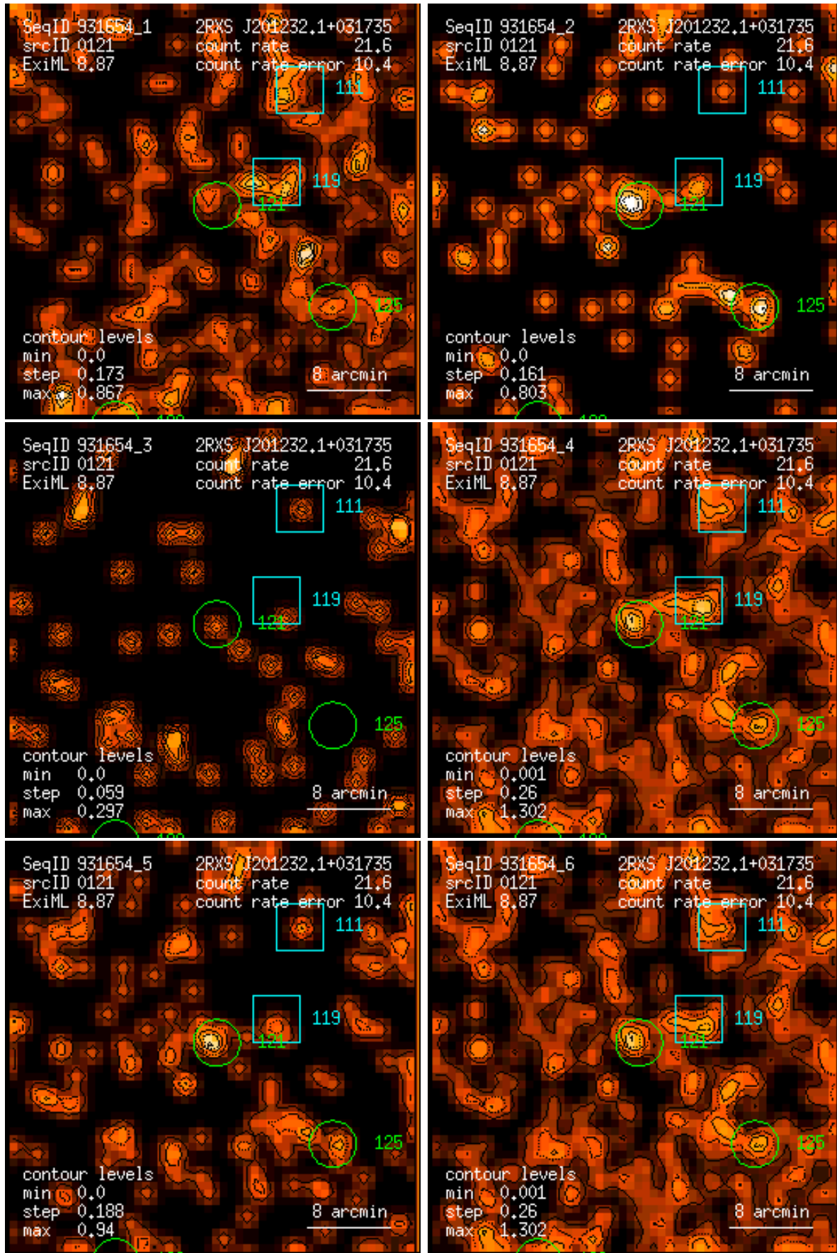
Figure 121: RASS 931654: detection 0121: band rate images, Gaussian filter: (1) PSPC channels 11 – 41, (2) 52 – 90, (3) 91 – 201, (4) 11 – 235, (5) 52 – 201, (6) 11 – 201. Broad band rates in counts/ks. Band rate contour levels in counts/ks/arcmin 2 .
