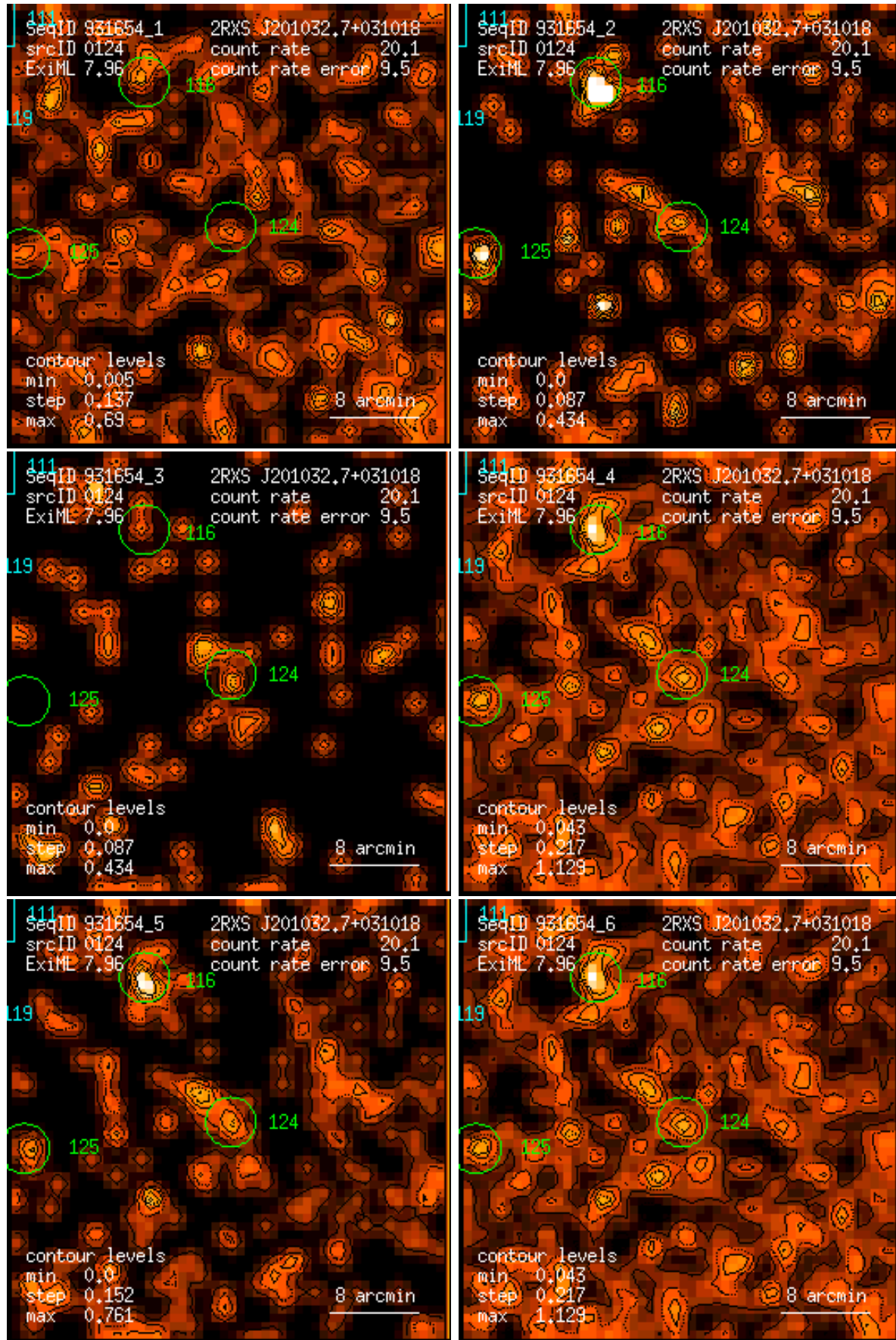
Figure 124: RASS 931654: detection 0124: band rate images, Gaussian filter: (1) PSPC channels 11 – 41, (2) 52 – 90, (3) 91 – 201, (4) 11 – 235, (5) 52 – 201, (6) 11 – 201. Broad band rates in counts/ks. Band rate contour levels in counts/ks/arcmin 2 .
