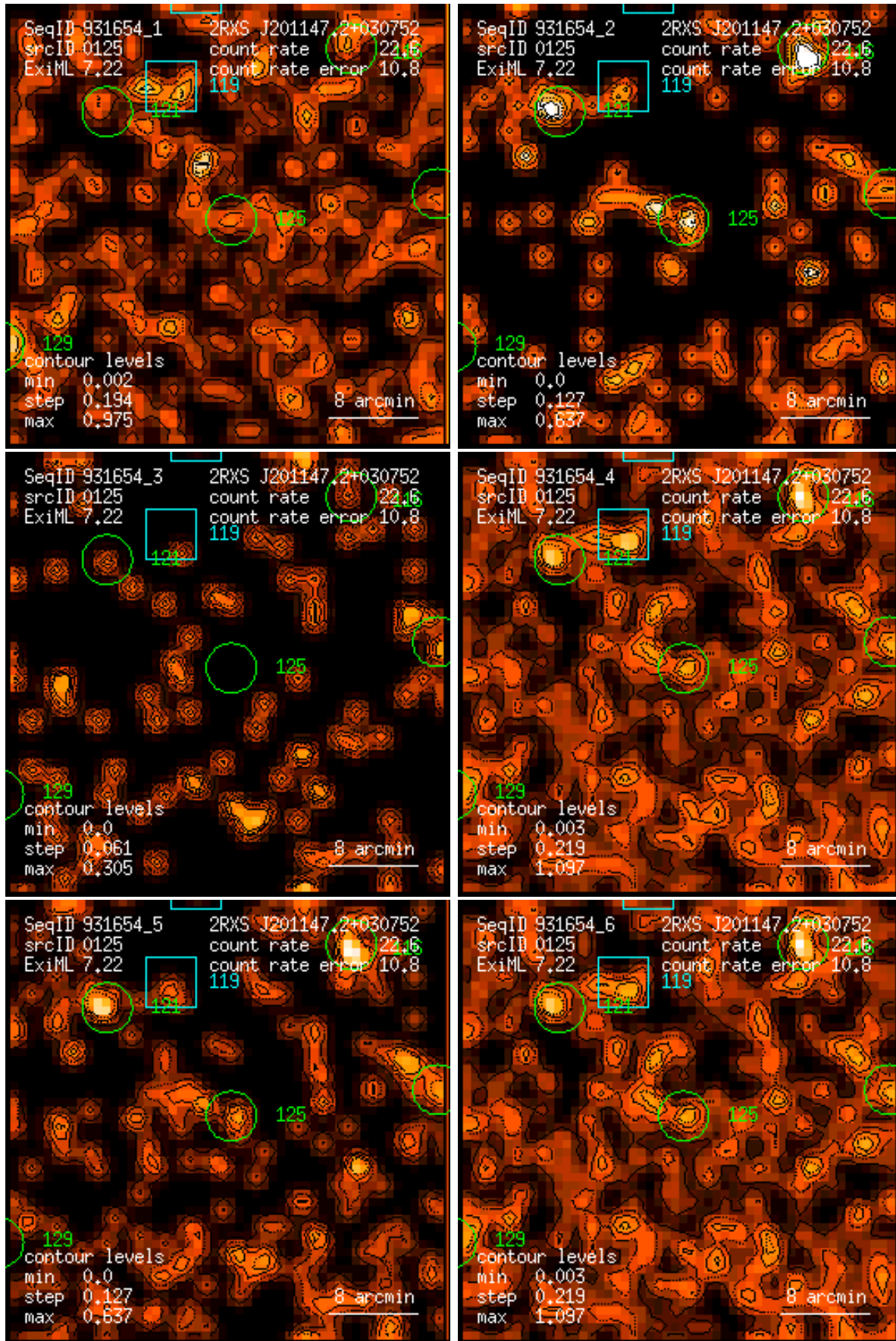
Figure 125: RASS 931654: detection 0125: band rate images, Gaussian filter: (1) PSPC channels 11 – 41, (2) 52 – 90, (3) 91 – 201, (4) 11 – 235, (5) 52 – 201, (6) 11 – 201. Broad band rates in counts/ks. Band rate contour levels in counts/ks/arcmin 2 .
