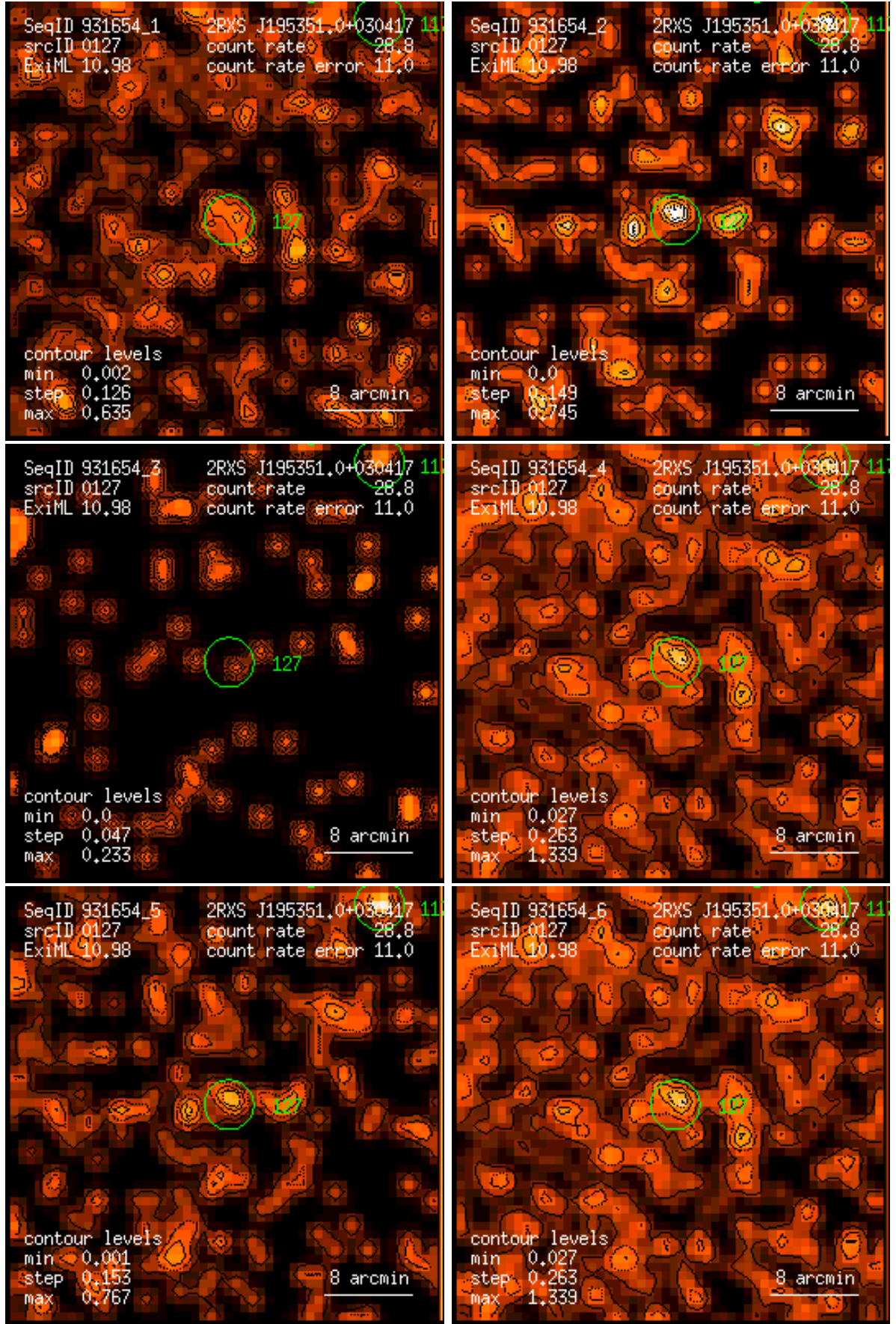
Figure 127: RASS 931654: detection 0127: band rate images, Gaussian filter: (1) PSPC channels 11 – 41, (2) 52 – 90, (3) 91 – 201, (4) 11 – 235, (5) 52 – 201, (6) 11 – 201. Broad band rates in counts/ks. Band rate contour levels in counts/ks/arcmin 2 .
