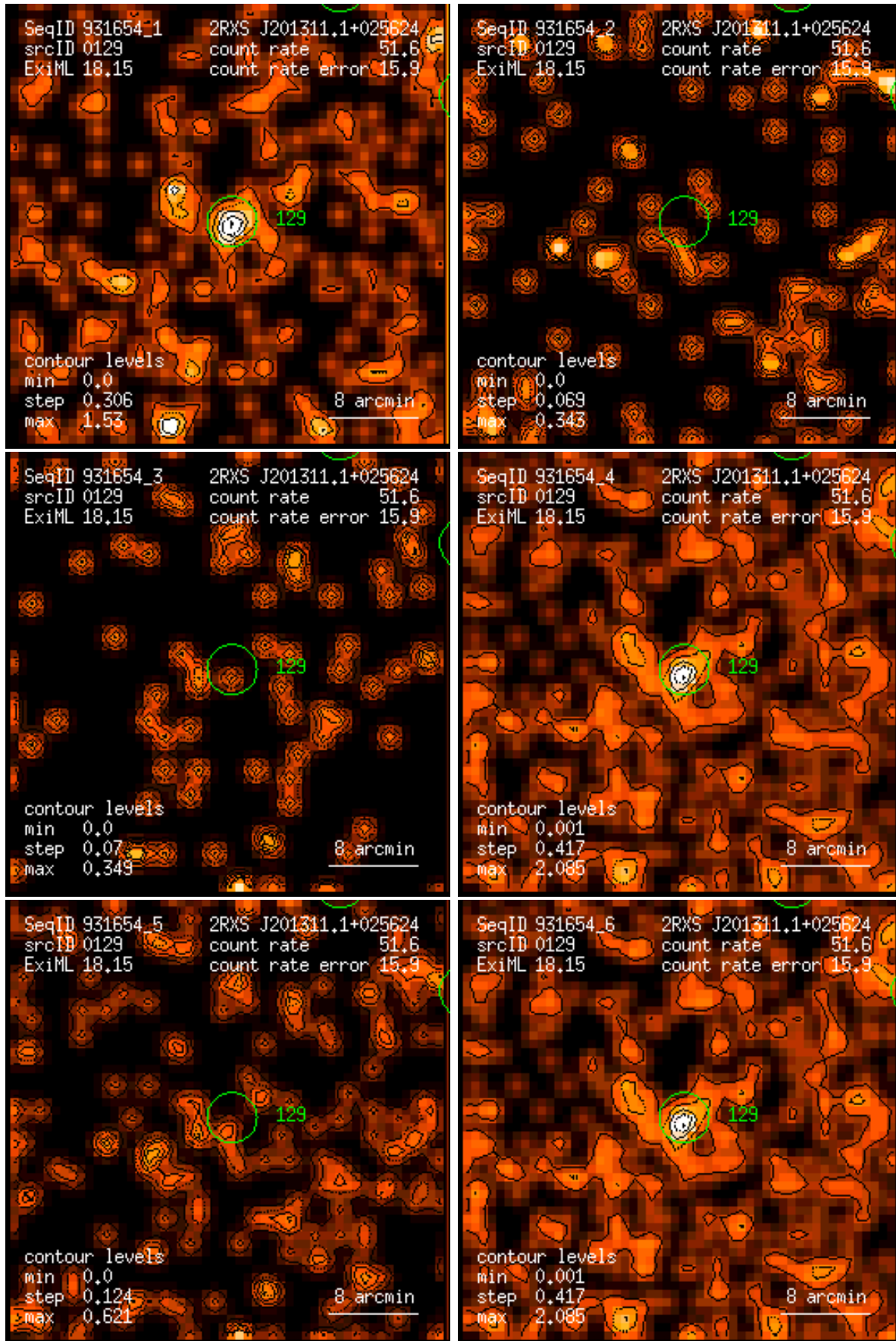
Figure 129: RASS 931654: detection 0129: band rate images, Gaussian filter: (1) PSPC channels 11 – 41, (2) 52 – 90, (3) 91 – 201, (4) 11 – 235, (5) 52 – 201, (6) 11 – 201. Broad band rates in counts/ks. Band rate contour levels in counts/ks/arcmin 2 .
