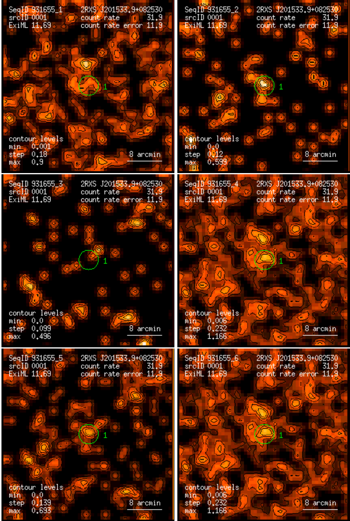
Figure 1: RASS 931655: detection 0001: band rate images, Gaussian filter: (1) PSPC channels 11 – 41, (2) 52 – 90, (3) 91 – 201, (4) 11 – 235, (5) 52 – 201, (6) 11 – 201. Broad band rates in counts/ks. Band rate contour levels in counts/ks/arcmin 2 .
