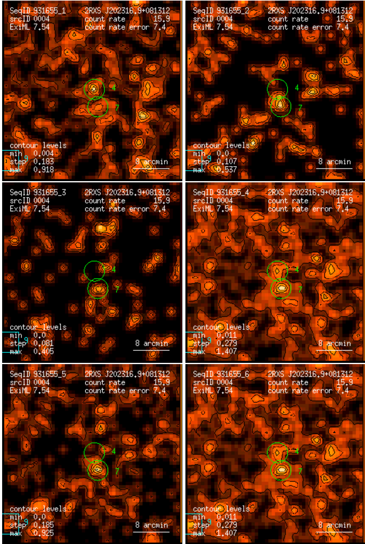
Figure 4: RASS 931655: detection 0004: band rate images, Gaussian filter: (1) PSPC channels 11 – 41, (2) 52 – 90, (3) 91 – 201, (4) 11 – 235, (5) 52 – 201, (6) 11 – 201. Broad band rates in counts/ks. Band rate contour levels in counts/ks/arcmin 2 .
