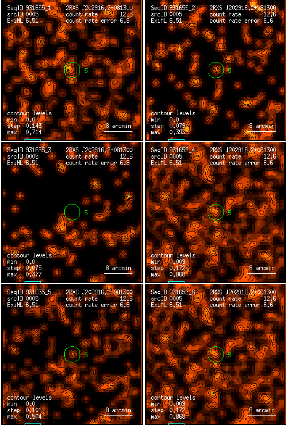
Figure 5: RASS 931655: detection 0005: band rate images, Gaussian filter: (1) PSPC channels 11 – 41, (2) 52 – 90, (3) 91 – 201, (4) 11 – 235, (5) 52 – 201, (6) 11 – 201. Broad band rates in counts/ks. Band rate contour levels in counts/ks/arcmin 2 .
