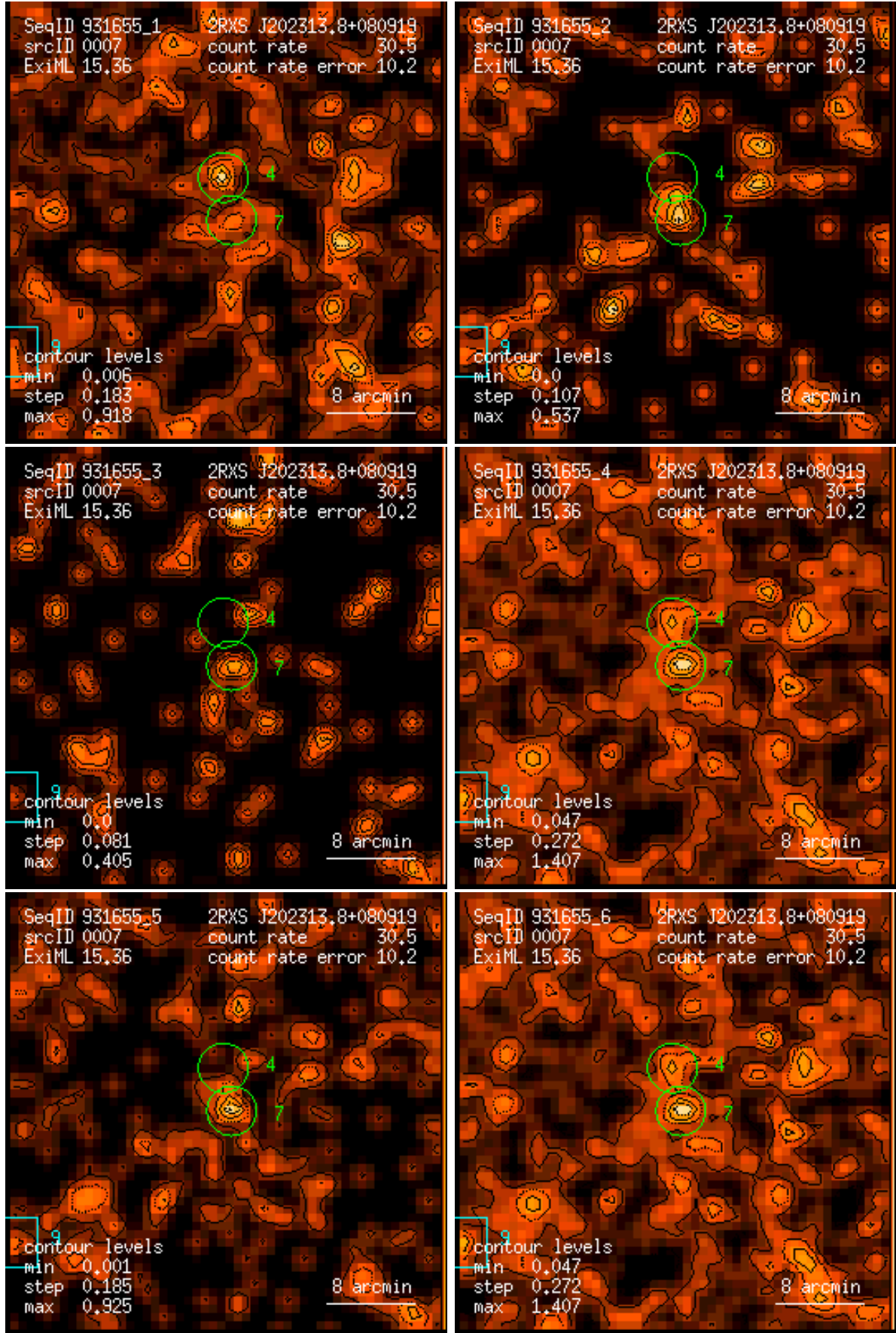
Figure 7: RASS 931655: detection 0007: band rate images, Gaussian filter: (1) PSPC channels 11 – 41, (2) 52 – 90, (3) 91 – 201, (4) 11 – 235, (5) 52 – 201, (6) 11 – 201. Broad band rates in counts/ks. Band rate contour levels in counts/ks/arcmin 2 .
