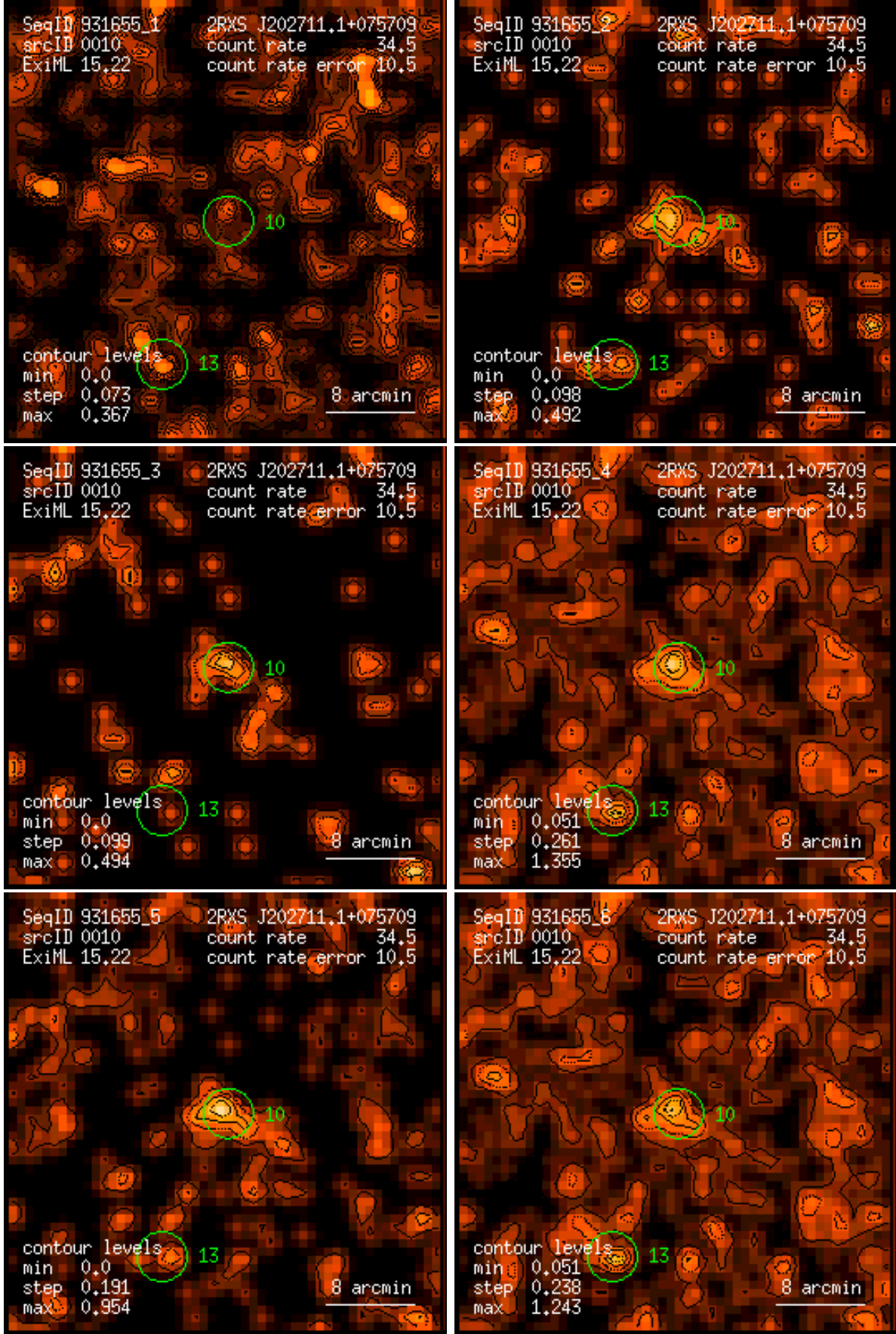
Figure 10: RASS 931655: detection 0010: band rate images, Gaussian filter: (1) PSPC channels 11 – 41, (2) 52 – 90, (3) 91 – 201, (4) 11 – 235, (5) 52 – 201, (6) 11 – 201. Broad band rates in counts/ks. Band rate contour levels in counts/ks/arcmin 2 .
