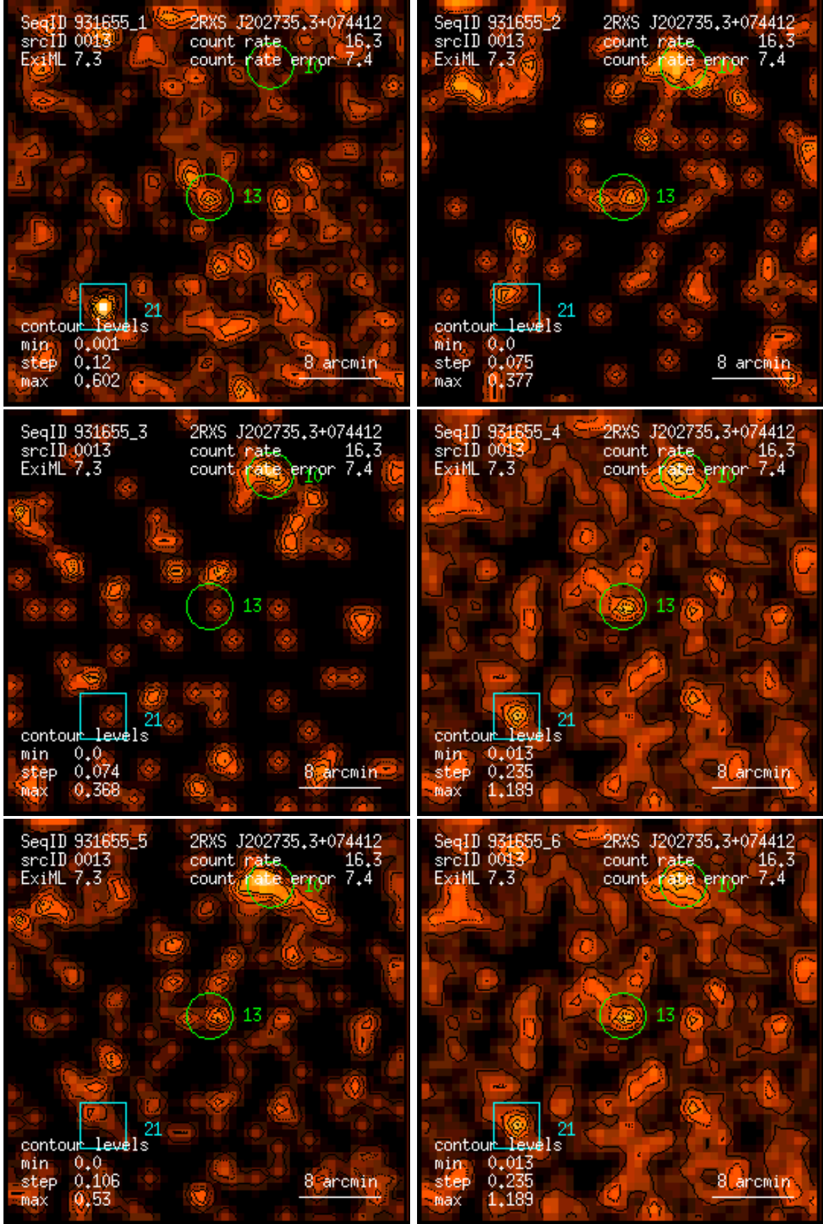
Figure 13: RASS 931655: detection 0013: band rate images, Gaussian filter: (1) PSPC channels 11 – 41, (2) 52 – 90, (3) 91 – 201, (4) 11 – 235, (5) 52 – 201, (6) 11 – 201. Broad band rates in counts/ks. Band rate contour levels in counts/ks/arcmin 2 .
