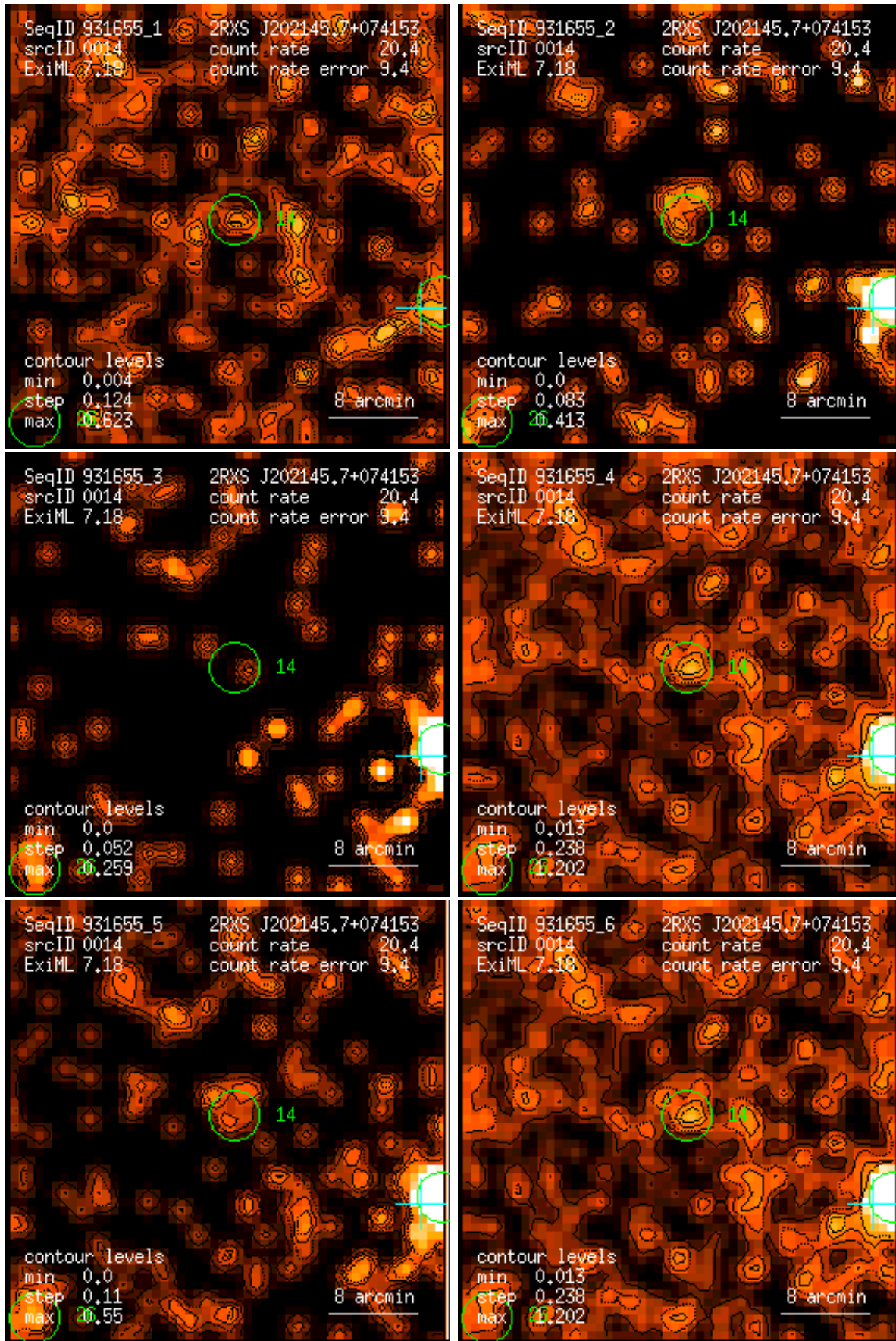
Figure 14: RASS 931655: detection 0014: band rate images, Gaussian filter: (1) PSPC channels 11 – 41, (2) 52 – 90, (3) 91 – 201, (4) 11 – 235, (5) 52 – 201, (6) 11 – 201. Broad band rates in counts/ks. Band rate contour levels in counts/ks/arcmin 2 .
