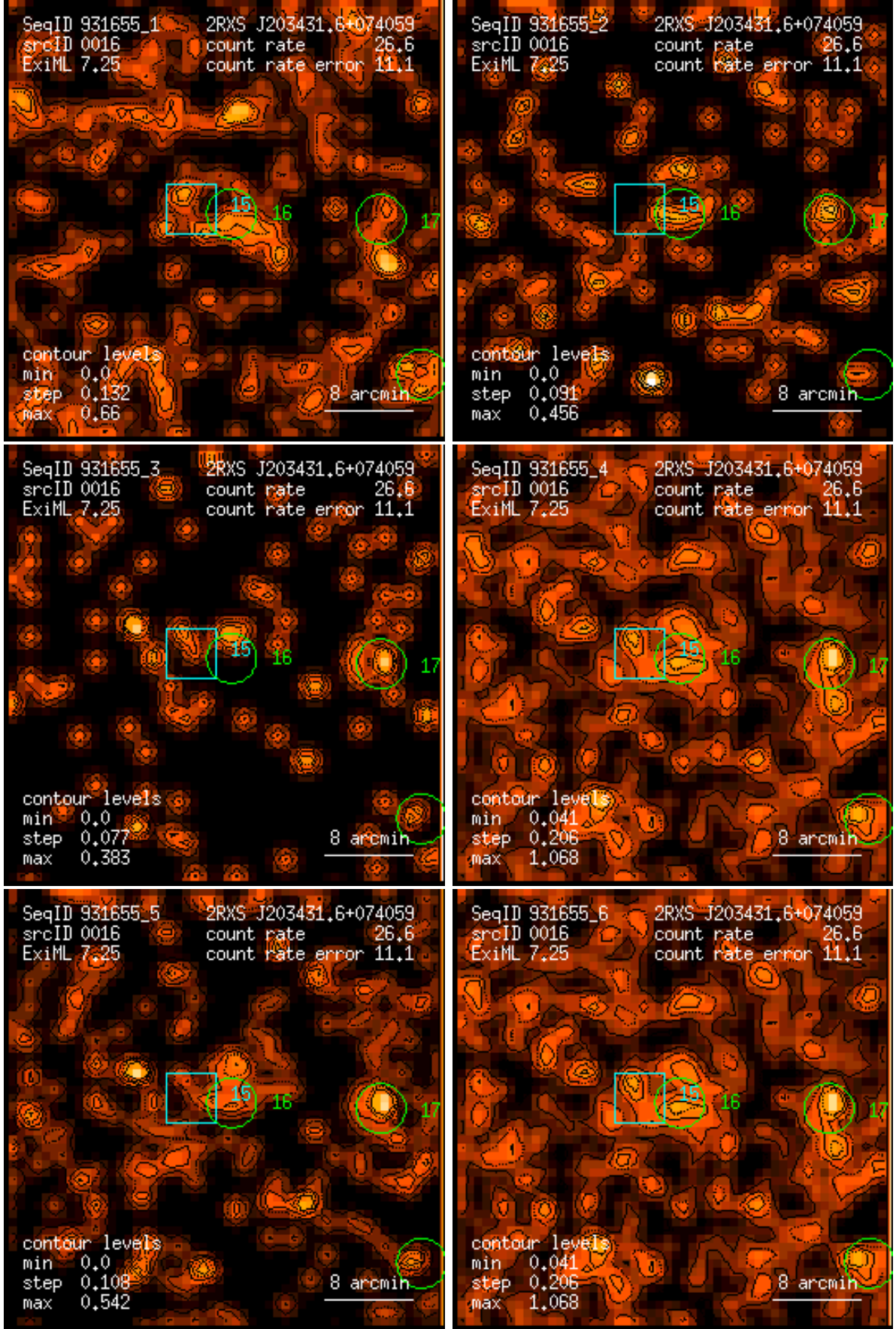
Figure 16: RASS 931655: detection 0016: band rate images, Gaussian filter: (1) PSPC channels 11 – 41, (2) 52 – 90, (3) 91 – 201, (4) 11 – 235, (5) 52 – 201, (6) 11 – 201. Broad band rates in counts/ks. Band rate contour levels in counts/ks/arcmin 2 .
