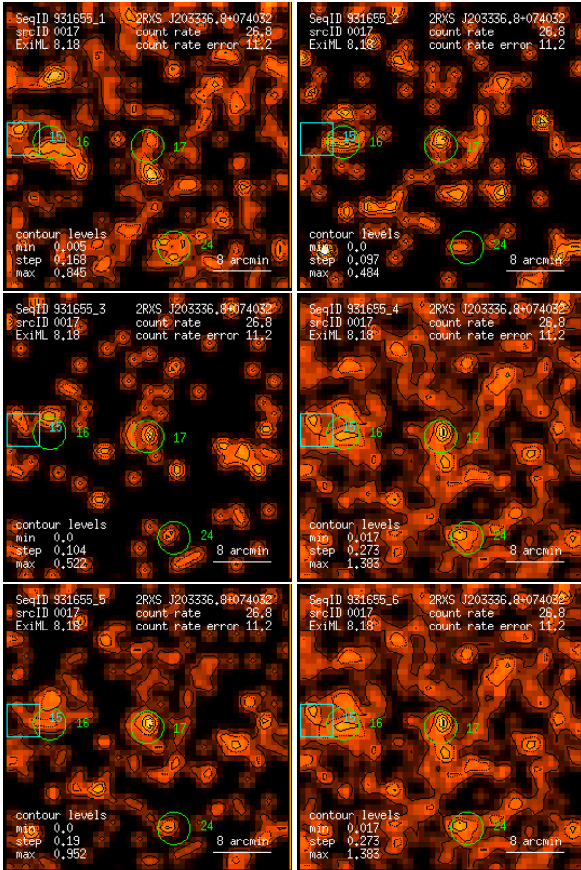
Figure 17: RASS 931655: detection 0017: band rate images, Gaussian filter: (1) PSPC channels 11 – 41, (2) 52 – 90, (3) 91 – 201, (4) 11 – 235, (5) 52 – 201, (6) 11 – 201. Broad band rates in counts/ks. Band rate contour levels in counts/ks/arcmin 2 .
