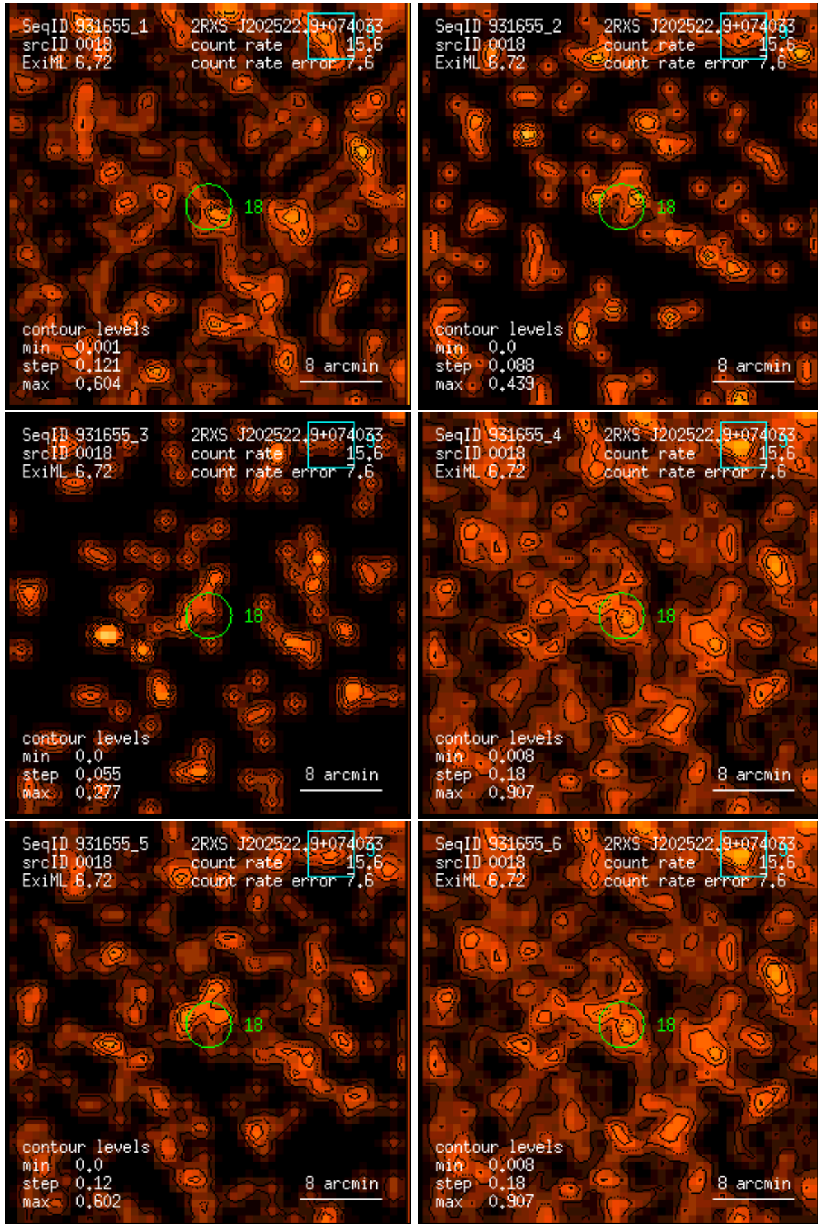
Figure 18: RASS 931655: detection 0018: band rate images, Gaussian filter: (1) PSPC channels 11 – 41, (2) 52 – 90, (3) 91 – 201, (4) 11 – 235, (5) 52 – 201, (6) 11 – 201. Broad band rates in counts/ks. Band rate contour levels in counts/ks/arcmin 2 .
