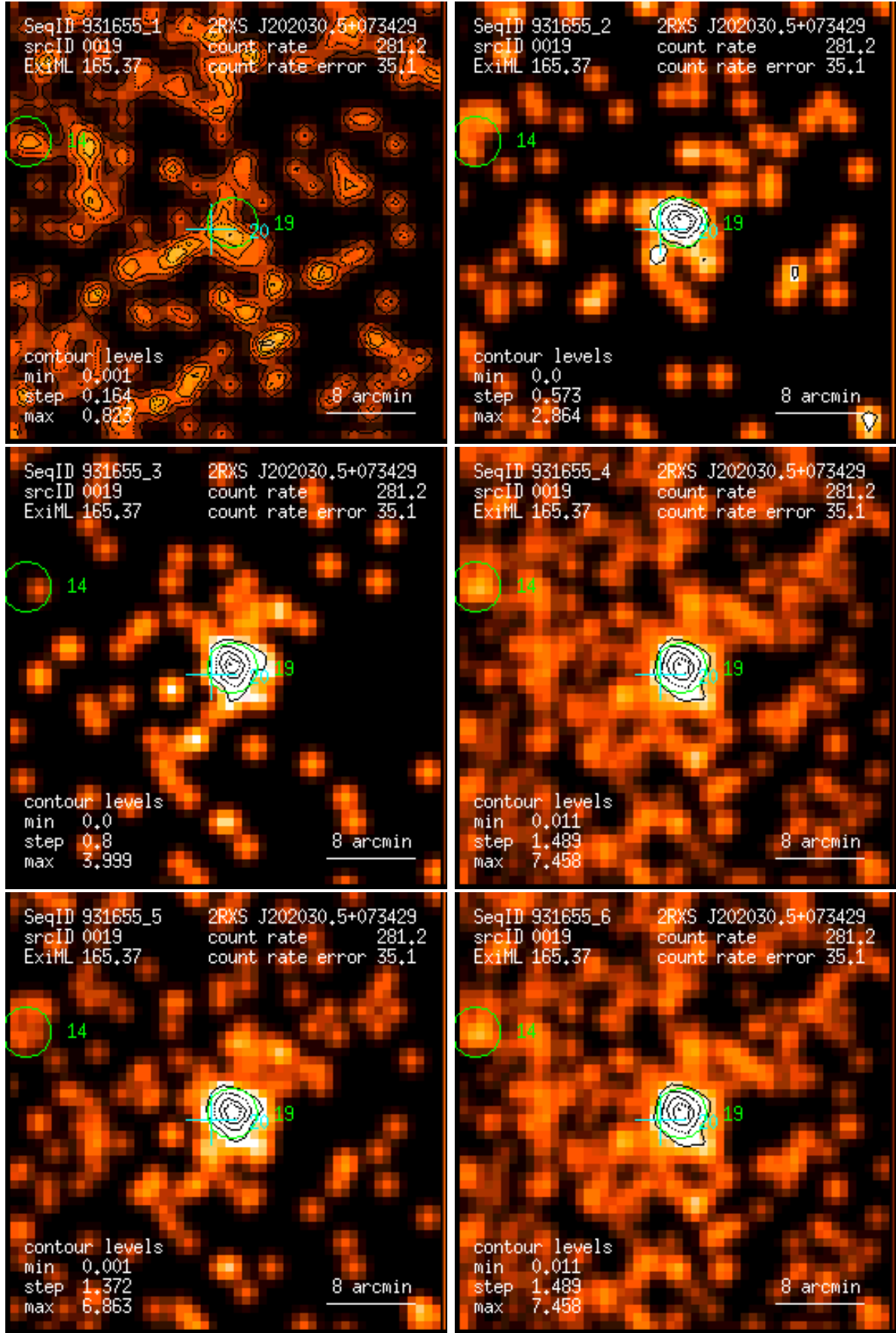
Figure 19: RASS 931655: detection 0019: band rate images, Gaussian filter: (1) PSPC channels 11 – 41, (2) 52 – 90, (3) 91 – 201, (4) 11 – 235, (5) 52 – 201, (6) 11 – 201. Broad band rates in counts/ks. Band rate contour levels in counts/ks/arcmin 2 .
